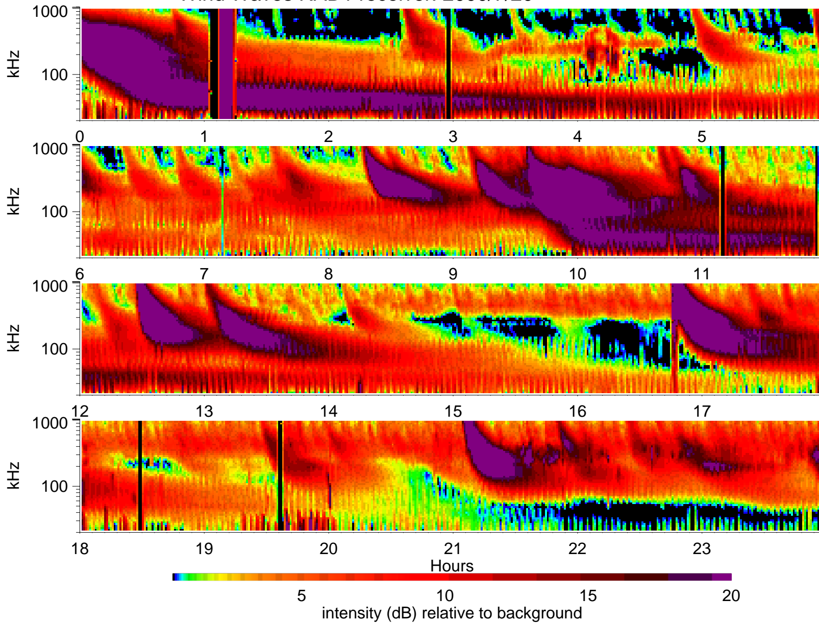
Wind Waves RAD1 receiver: 2000/7/20
