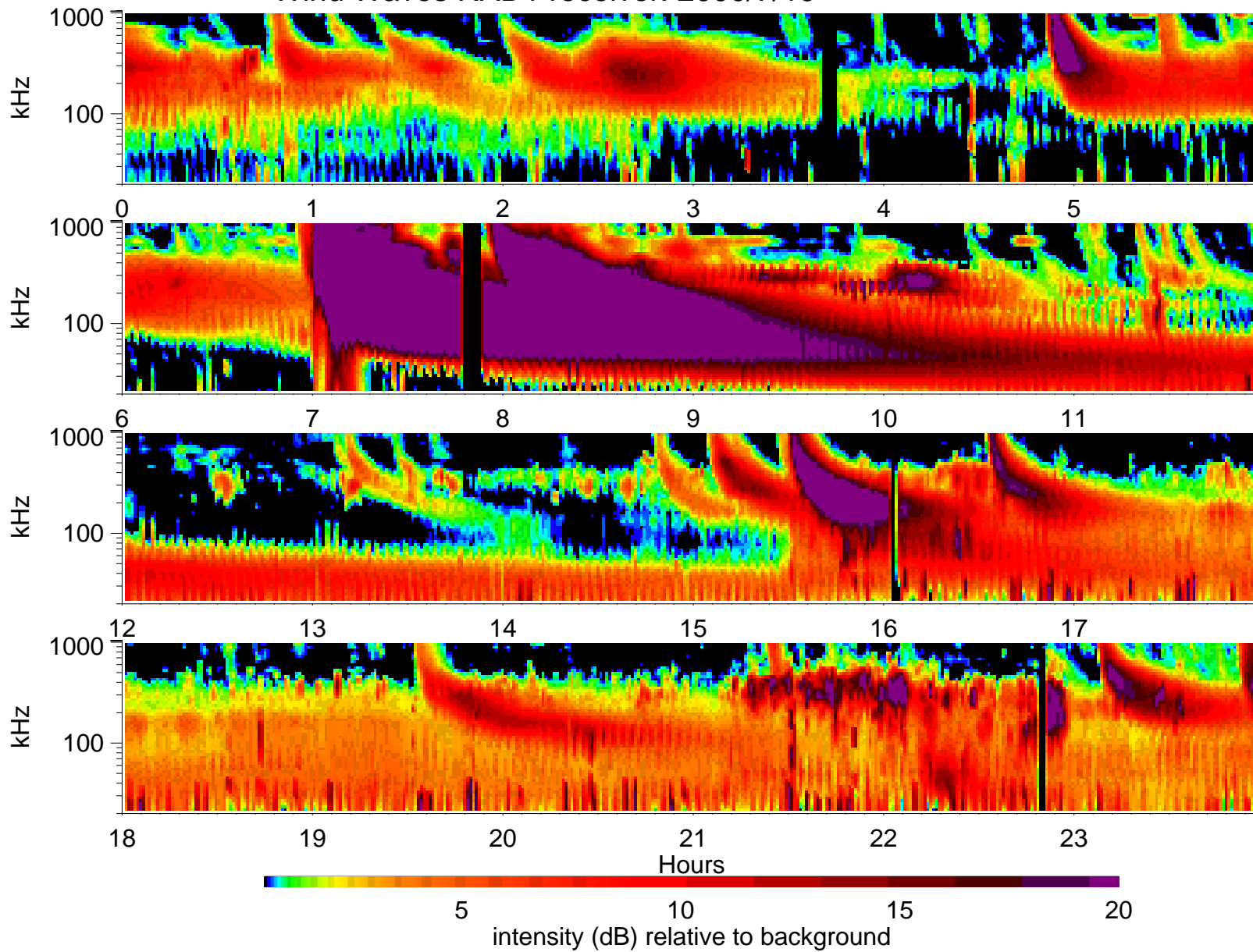
Wind Waves RAD1 receiver: 2000/7/19
