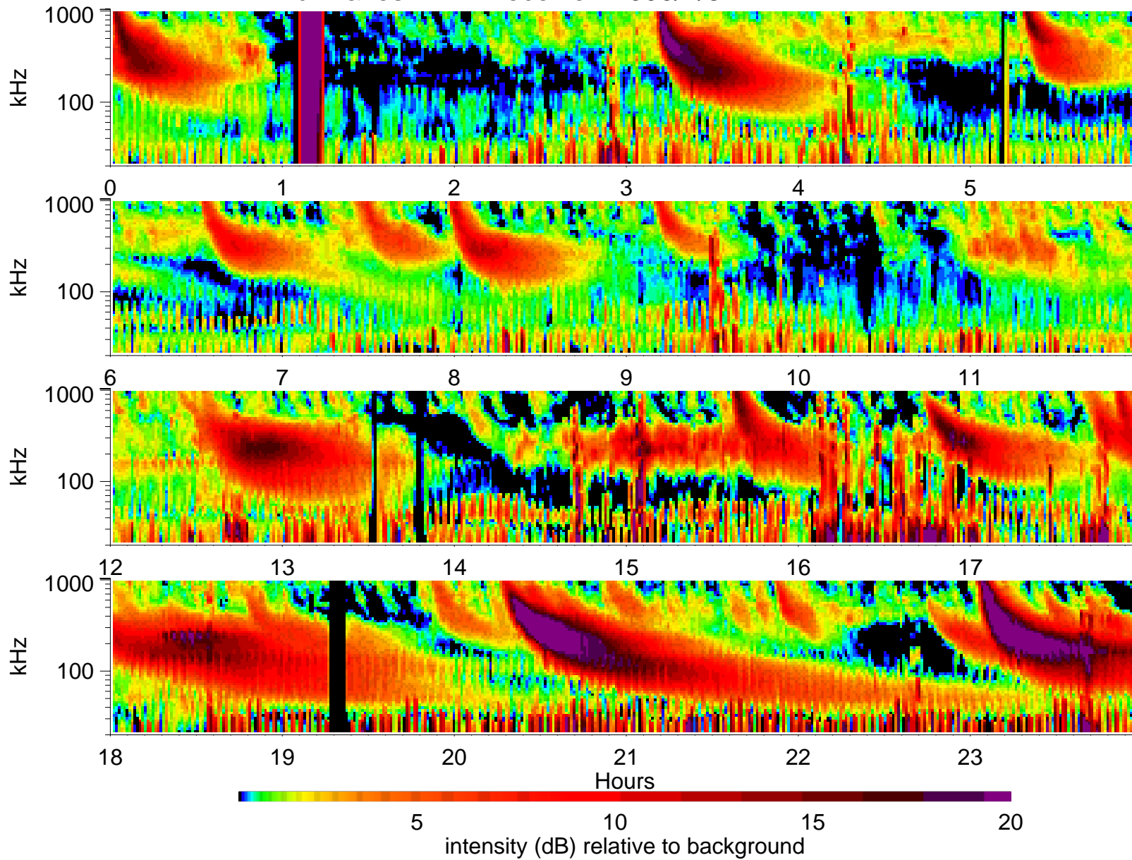
Wind Waves RAD1 receiver: 2000/7/8
