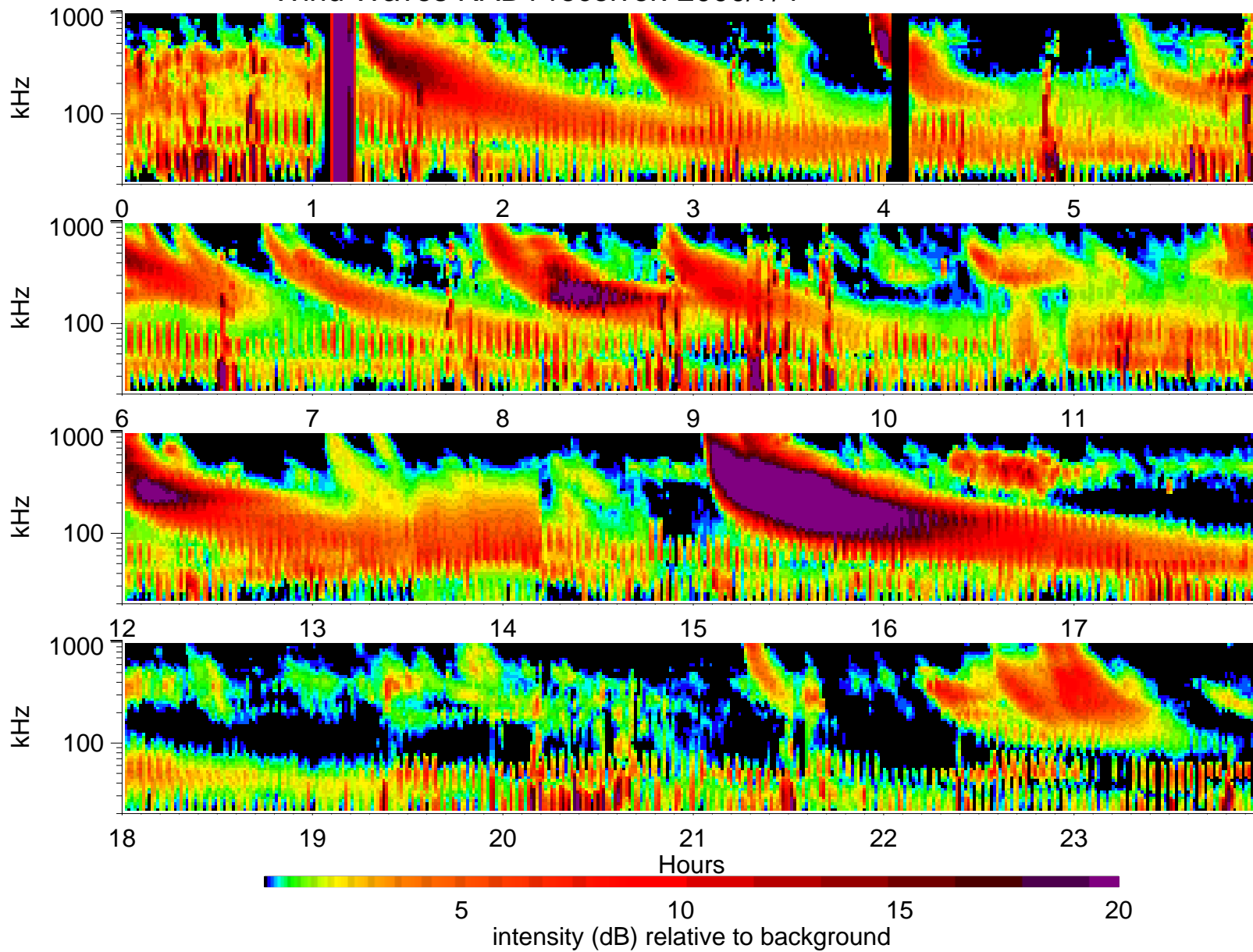
Wind Waves RAD1 receiver: 2000/7/4
