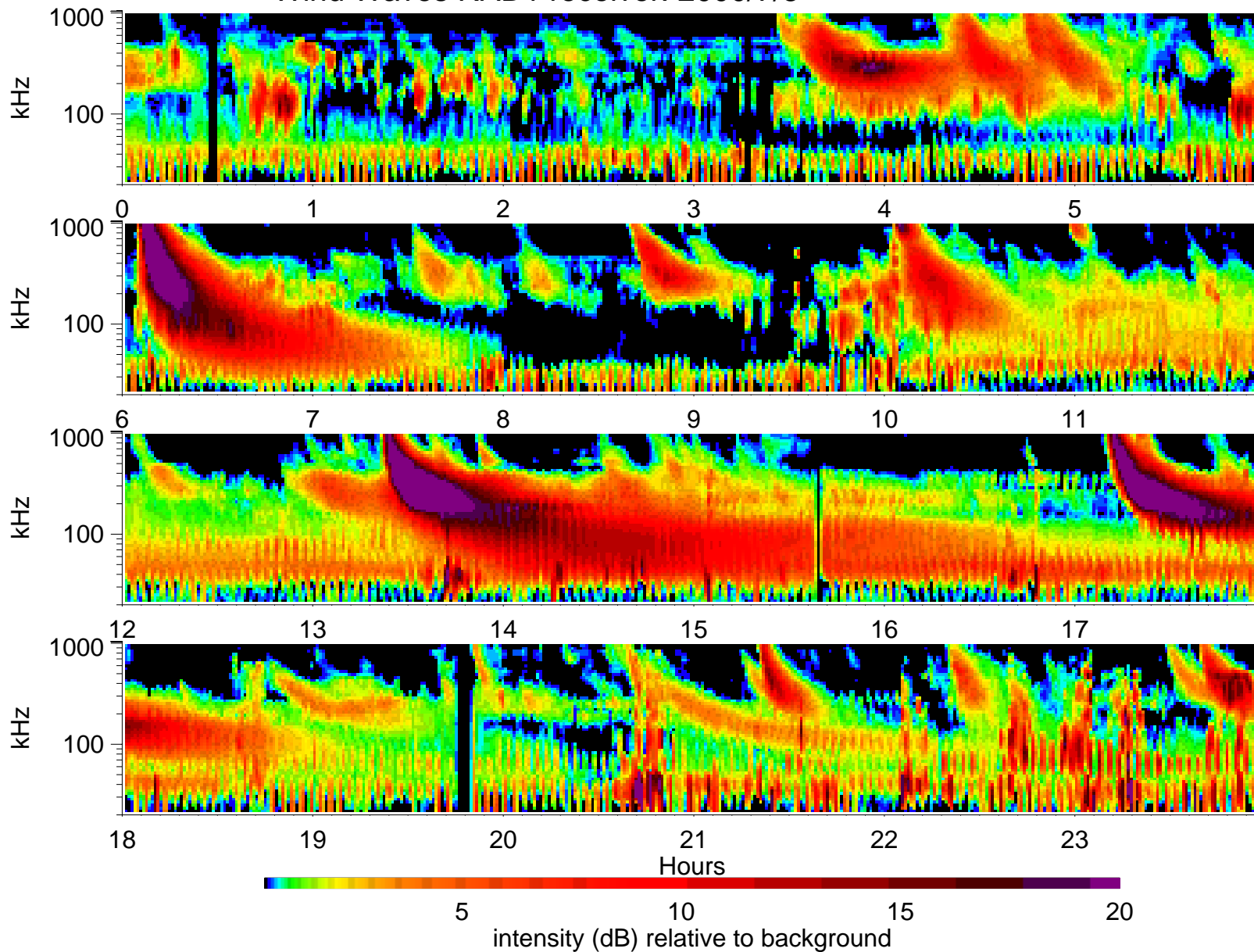
Wind Waves RAD1 receiver: 2000/7/3
