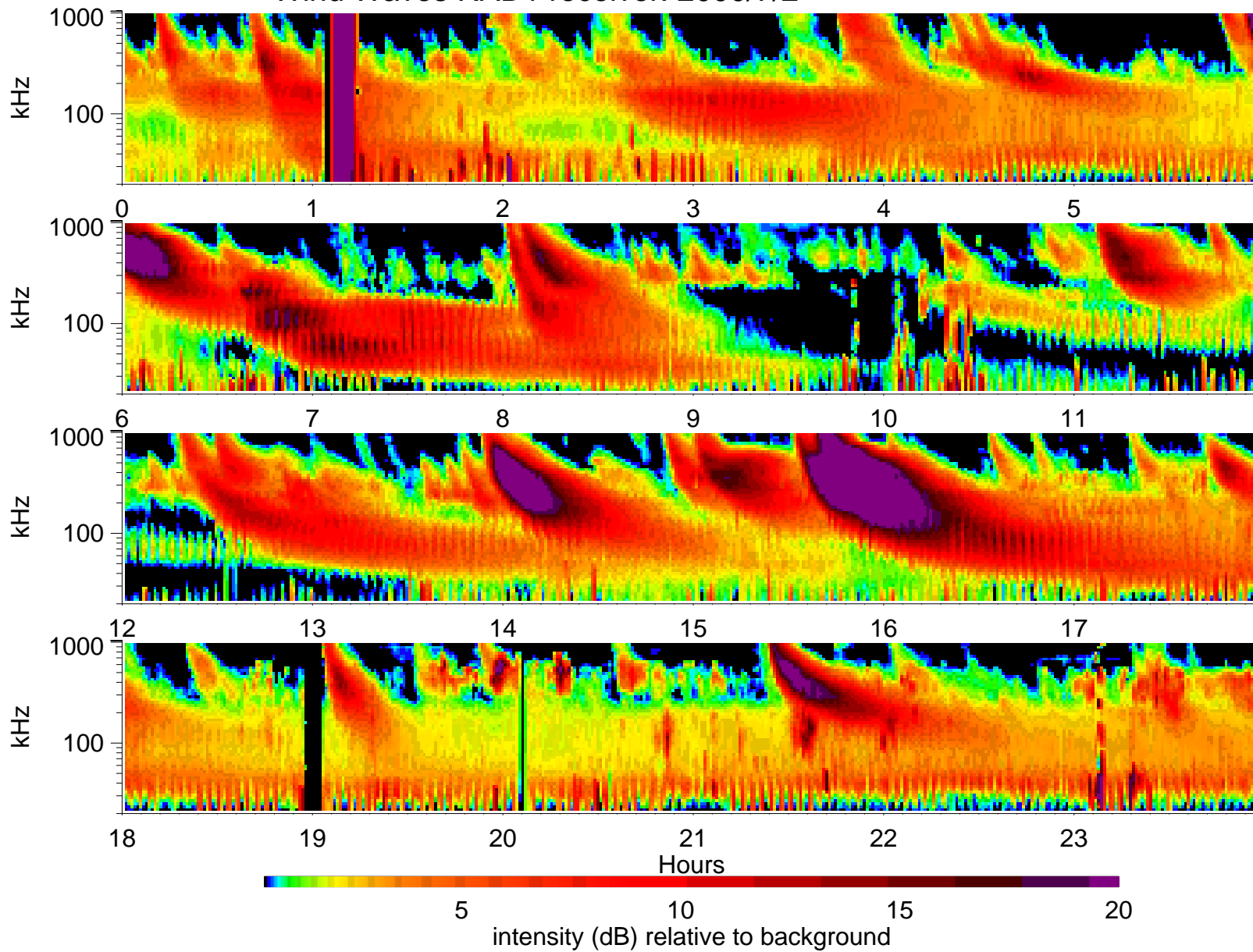
Wind Waves RAD1 receiver: 2000/7/2
