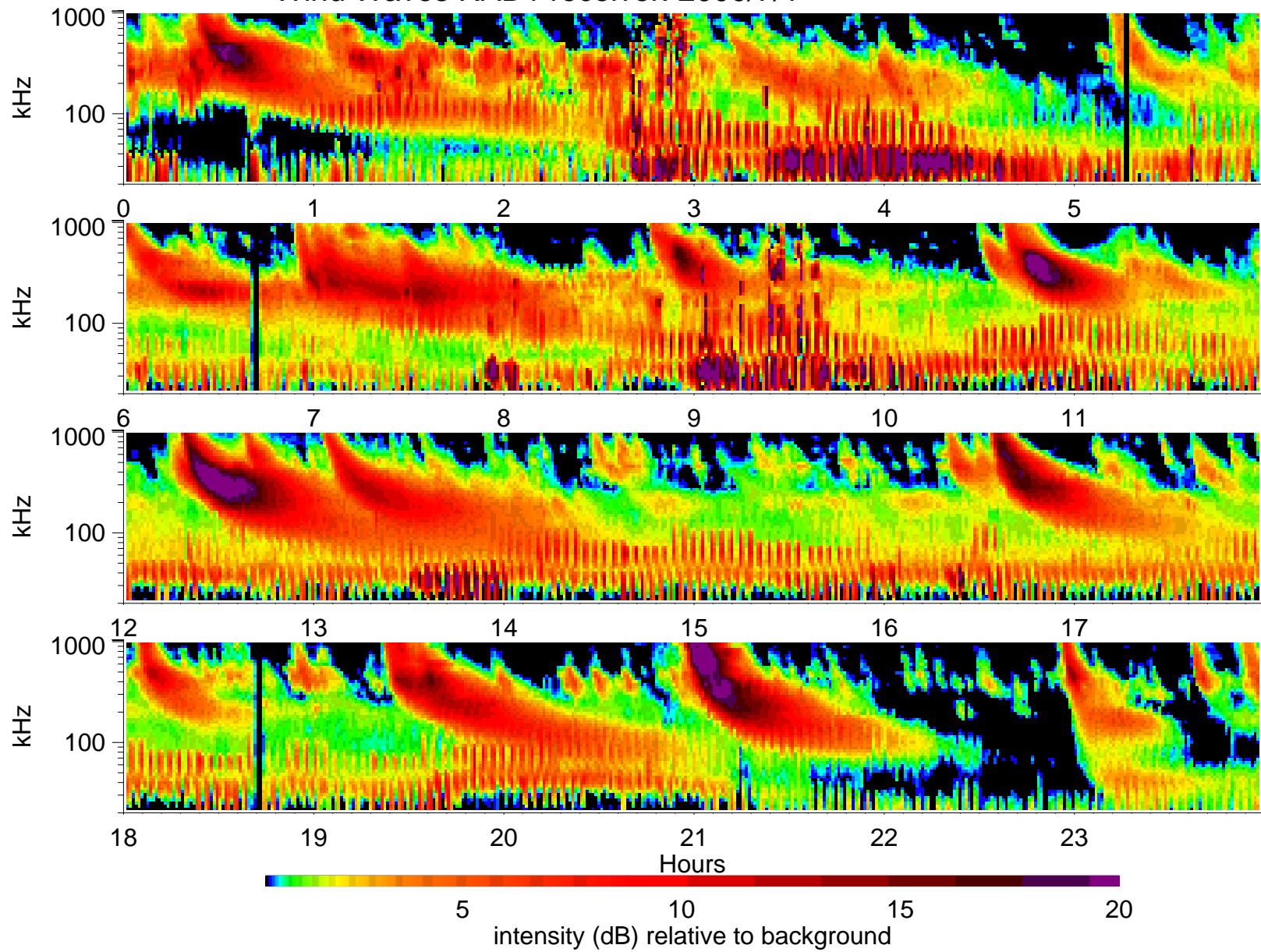
Wind Waves RAD1 receiver: 2000/7/1
