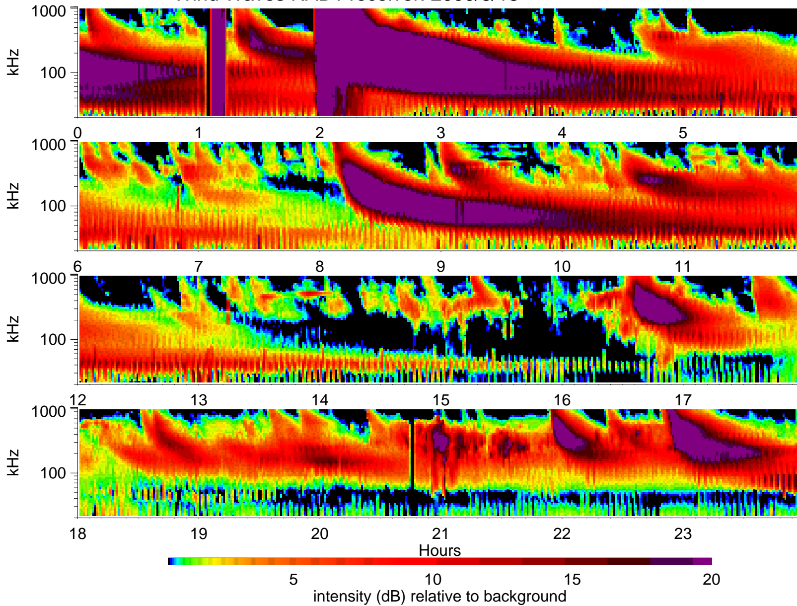
Wind Waves RAD1 receiver: 2000/6/18
