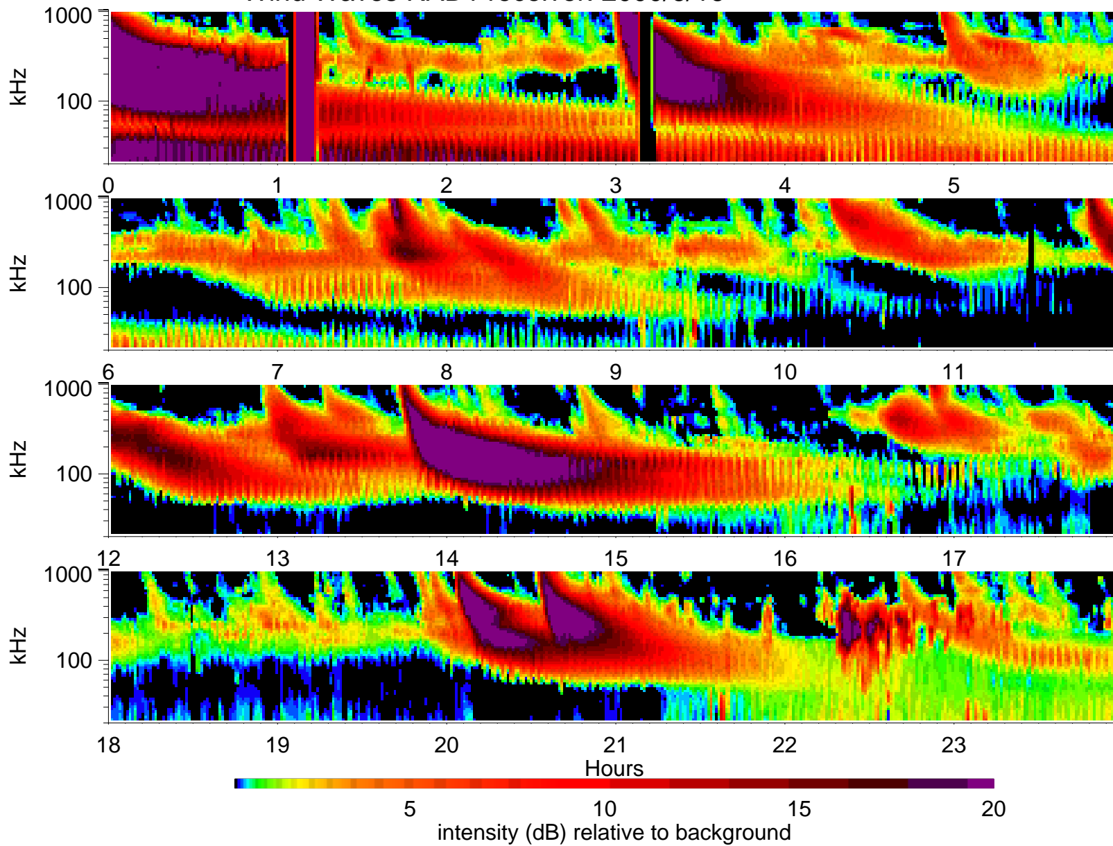
Wind Waves RAD1 receiver: 2000/6/16
