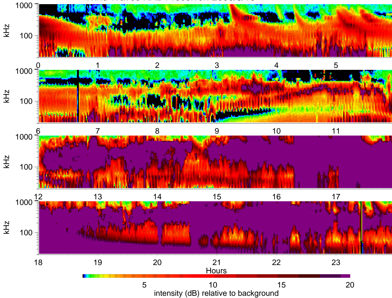
Wind Waves RAD1 receiver: 2000/6/10
