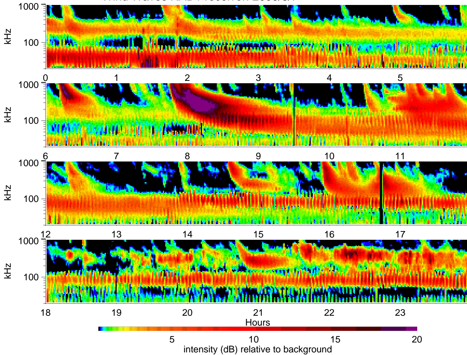
Wind Waves RAD1 receiver: 2000/6/7
