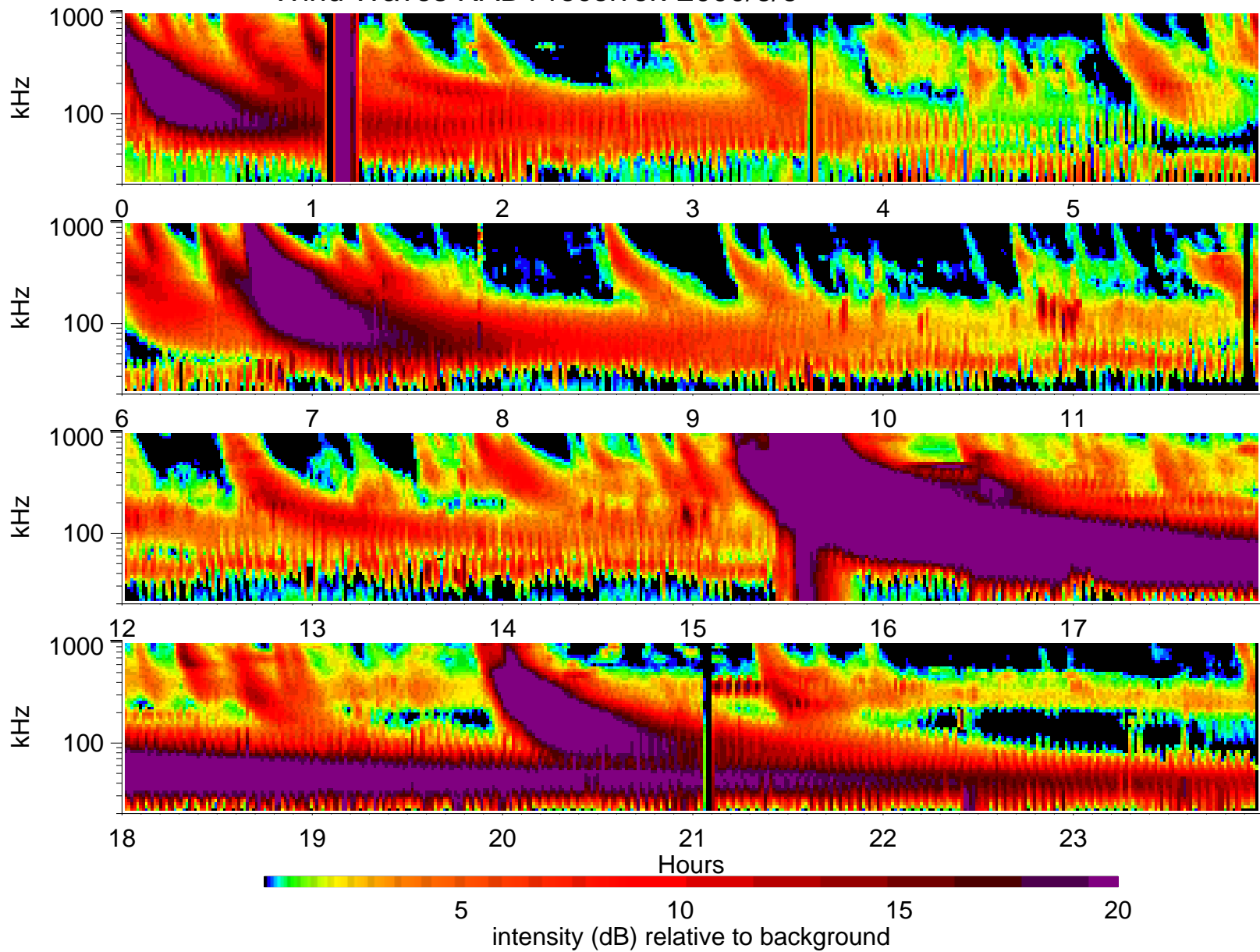
Wind Waves RAD1 receiver: 2000/6/6
