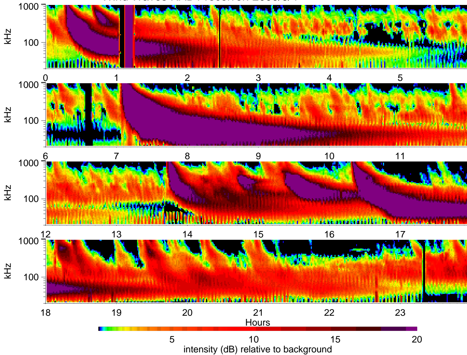
Wind Waves RAD1 receiver: 2000/6/4
