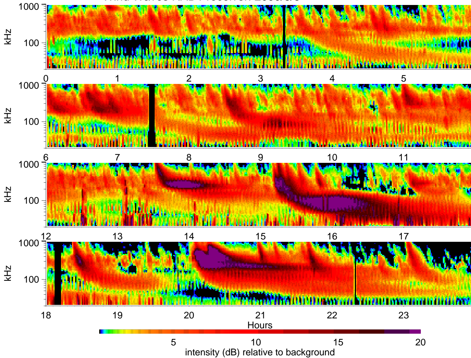
Wind Waves RAD1 receiver: 2000/6/3
