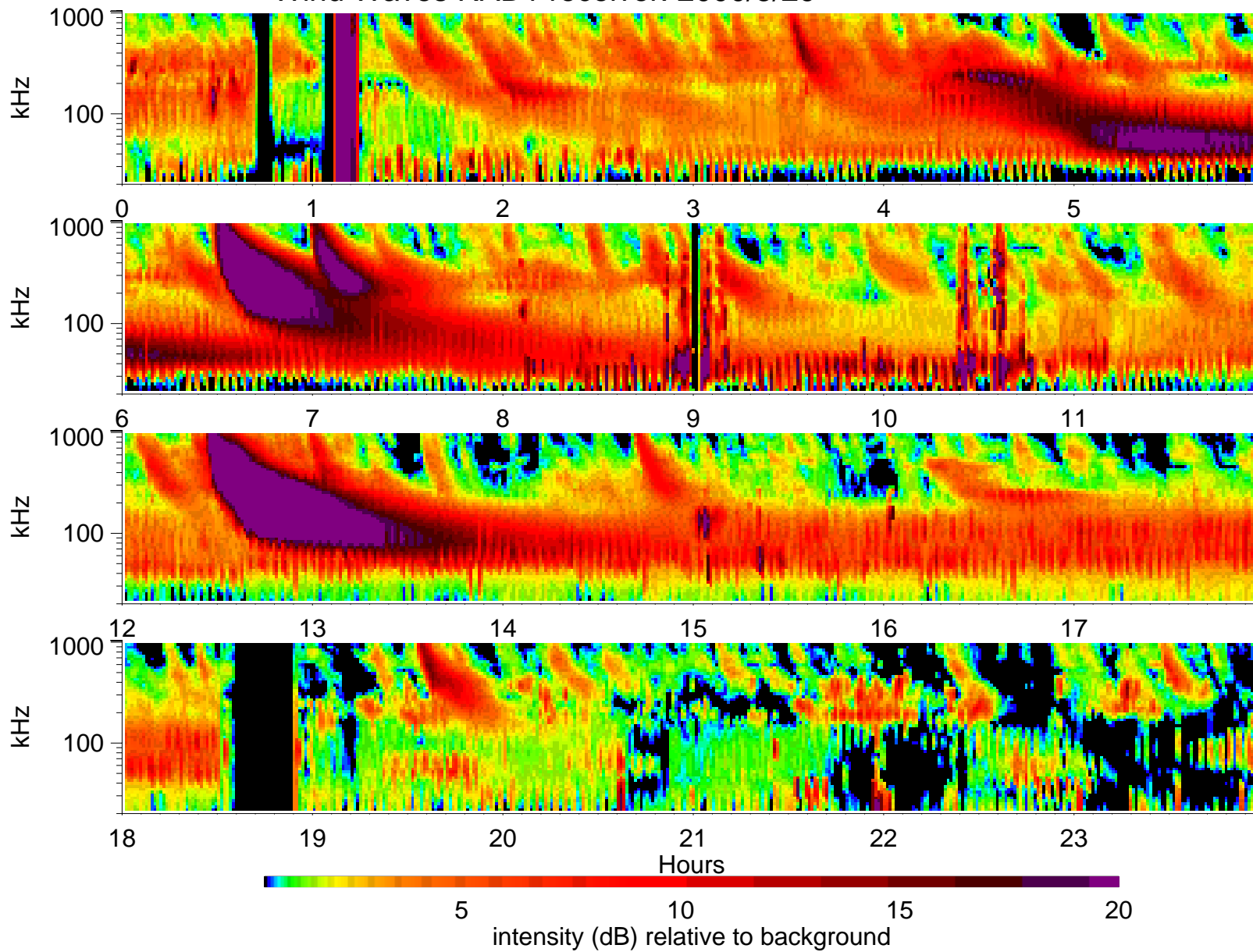
Wind Waves RAD1 receiver: 2000/5/29
