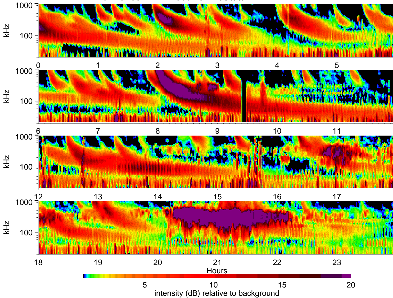
Wind Waves RAD1 receiver: 2000/5/27
