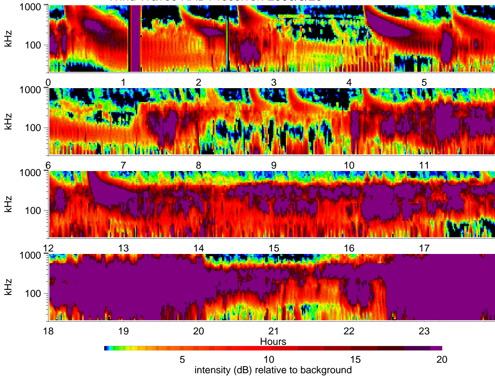
Wind Waves RAD1 receiver: 2000/5/25
