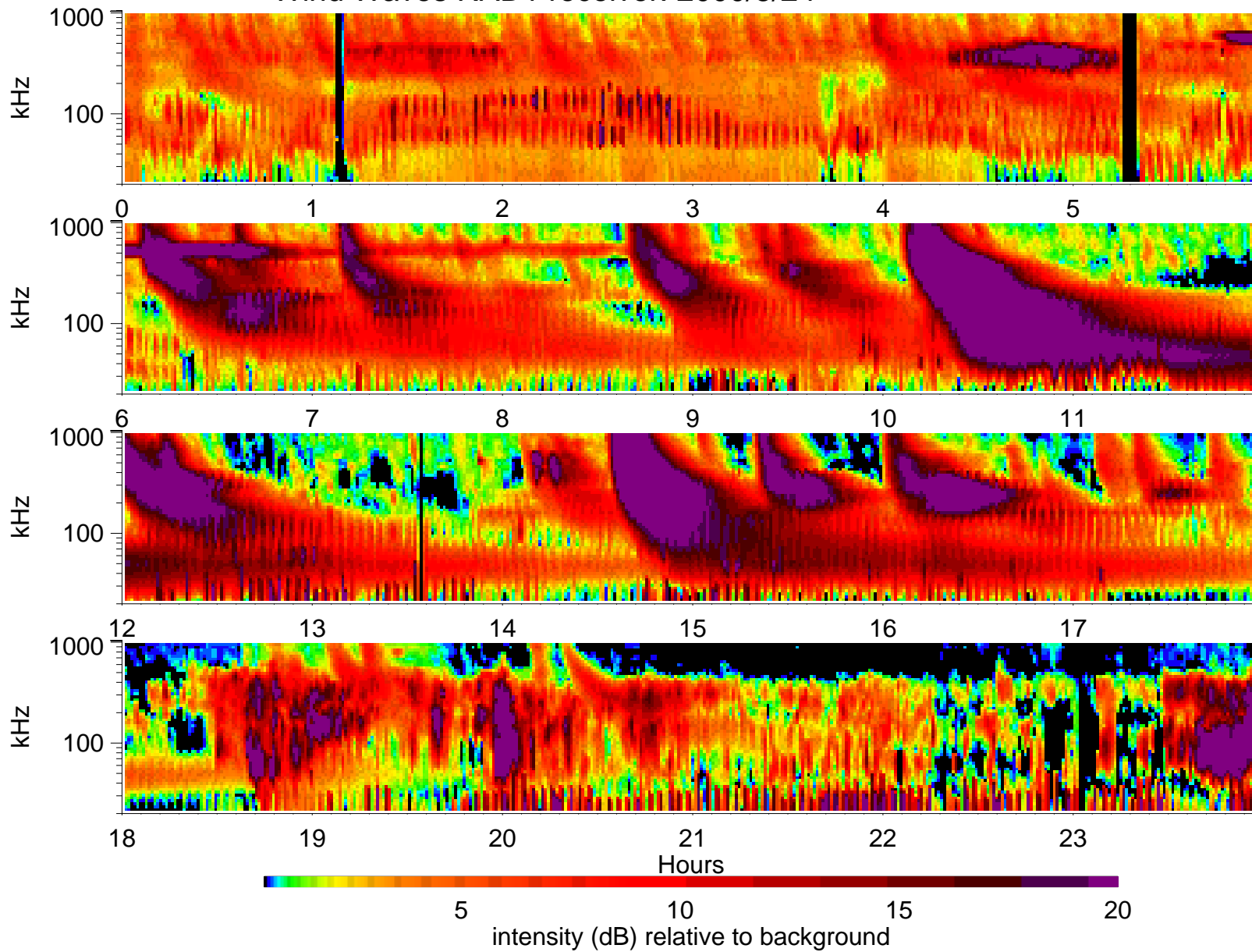
Wind Waves RAD1 receiver: 2000/5/24
