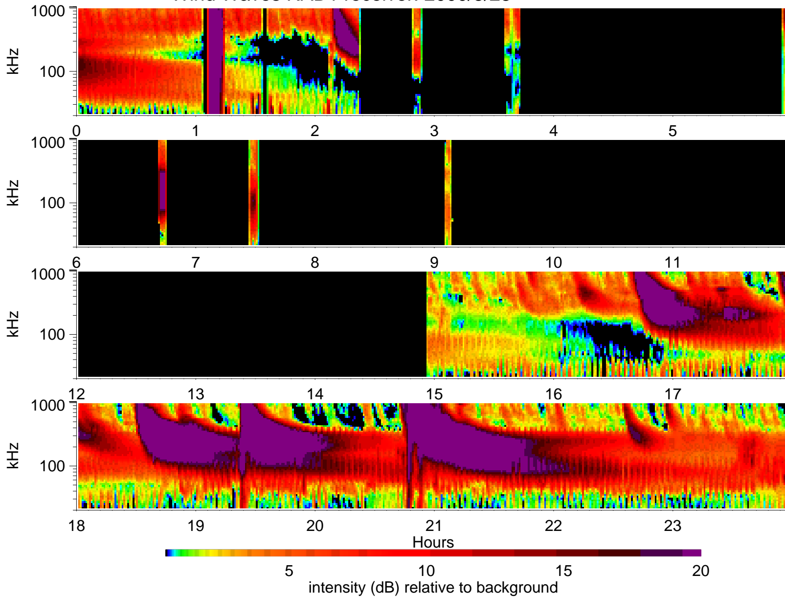
Wind Waves RAD1 receiver: 2000/5/23
