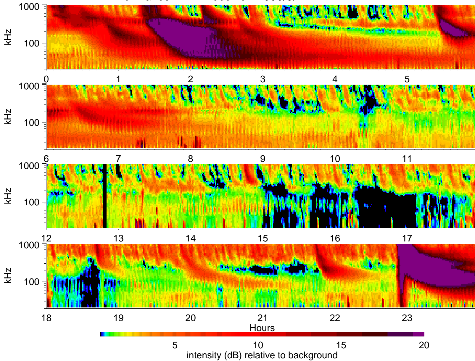
Wind Waves RAD1 receiver: 2000/5/22
