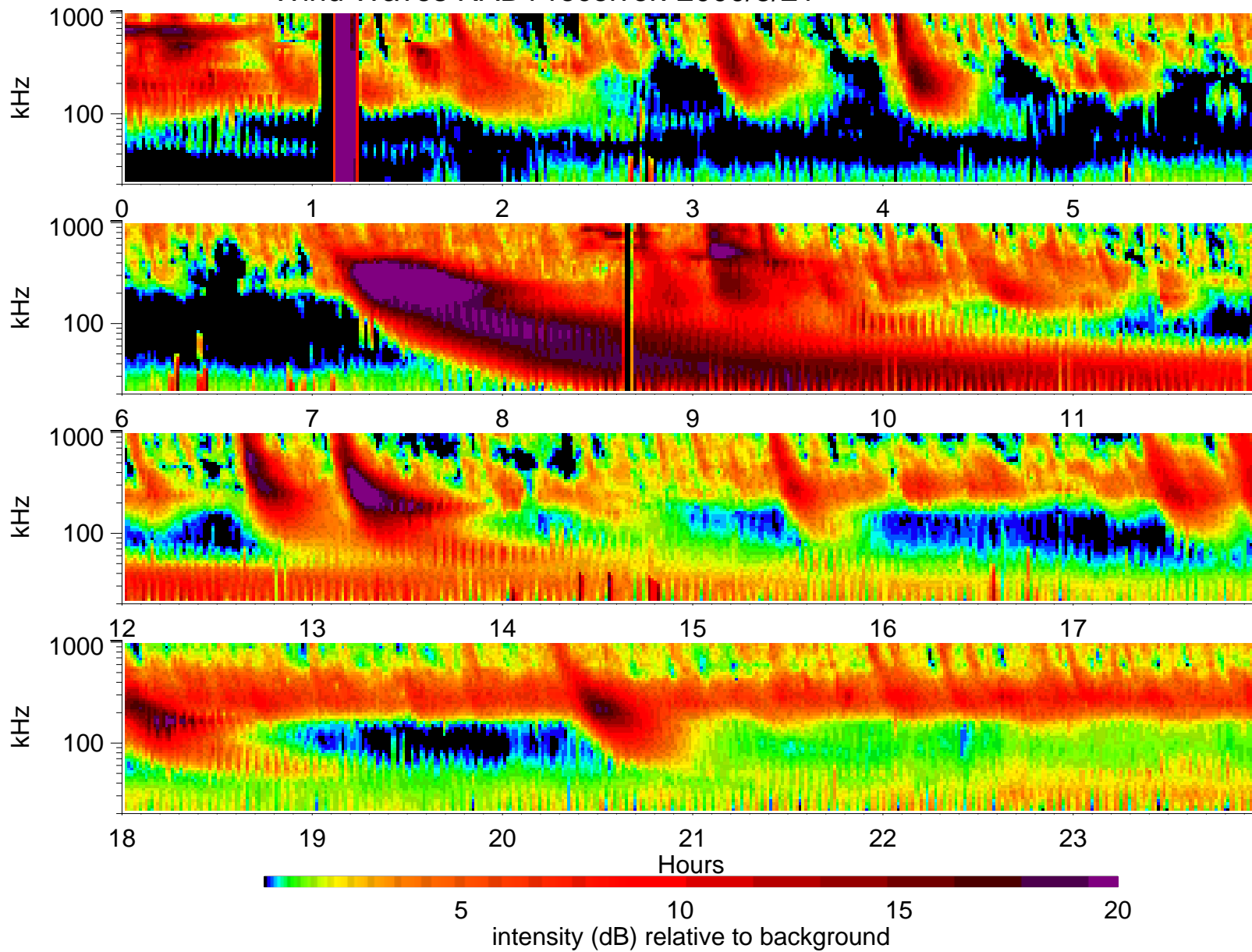
Wind Waves RAD1 receiver: 2000/5/21
