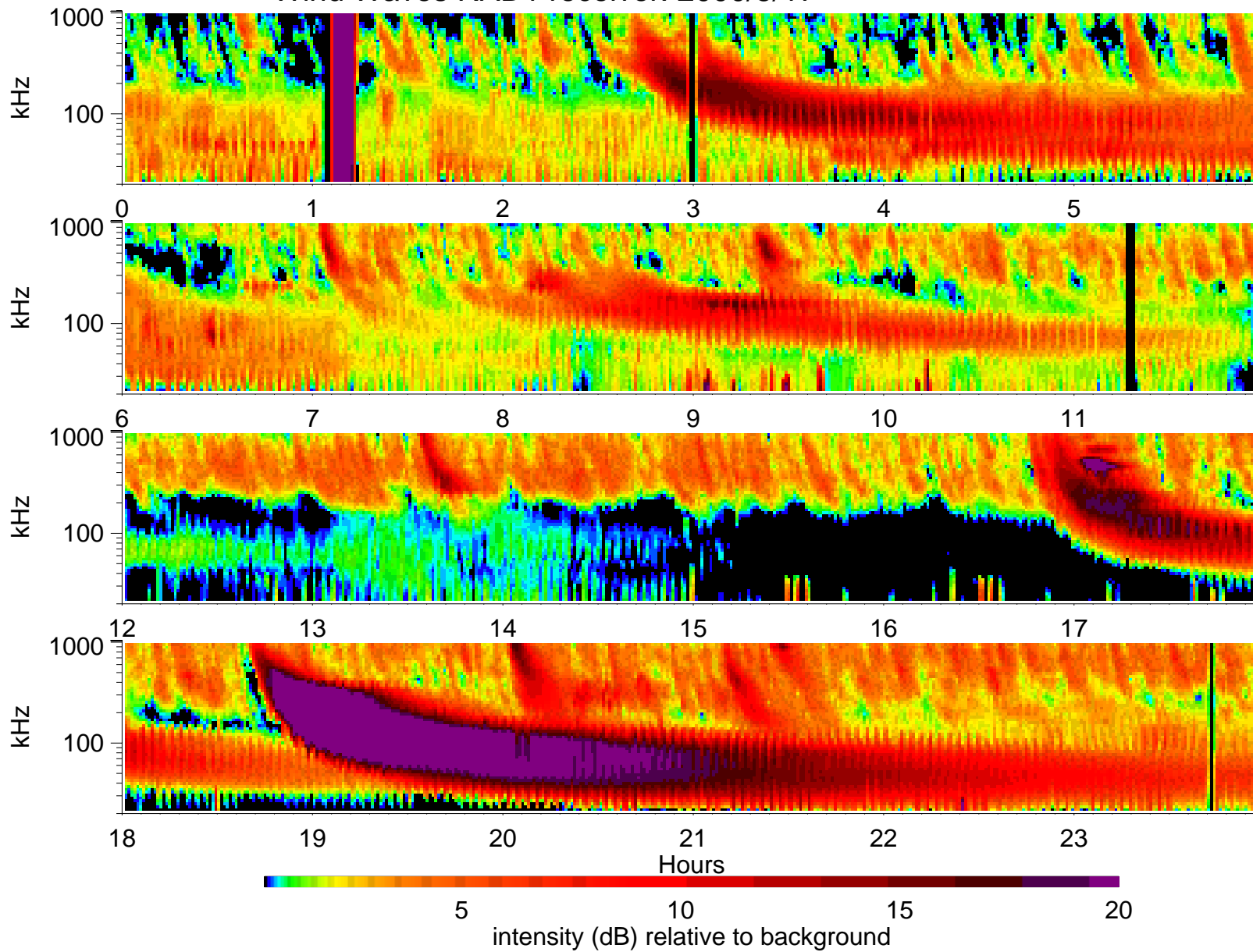
Wind Waves RAD1 receiver: 2000/5/17
