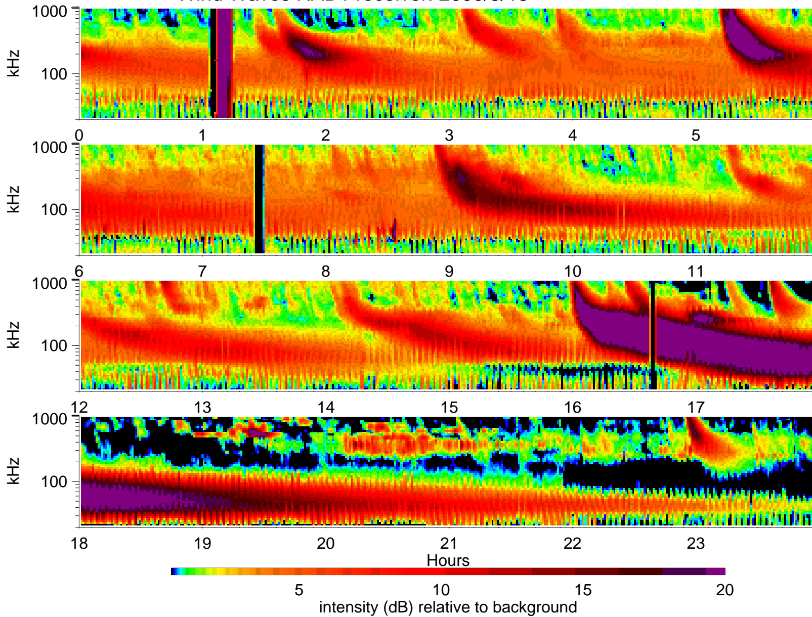
Wind Waves RAD1 receiver: 2000/5/15
