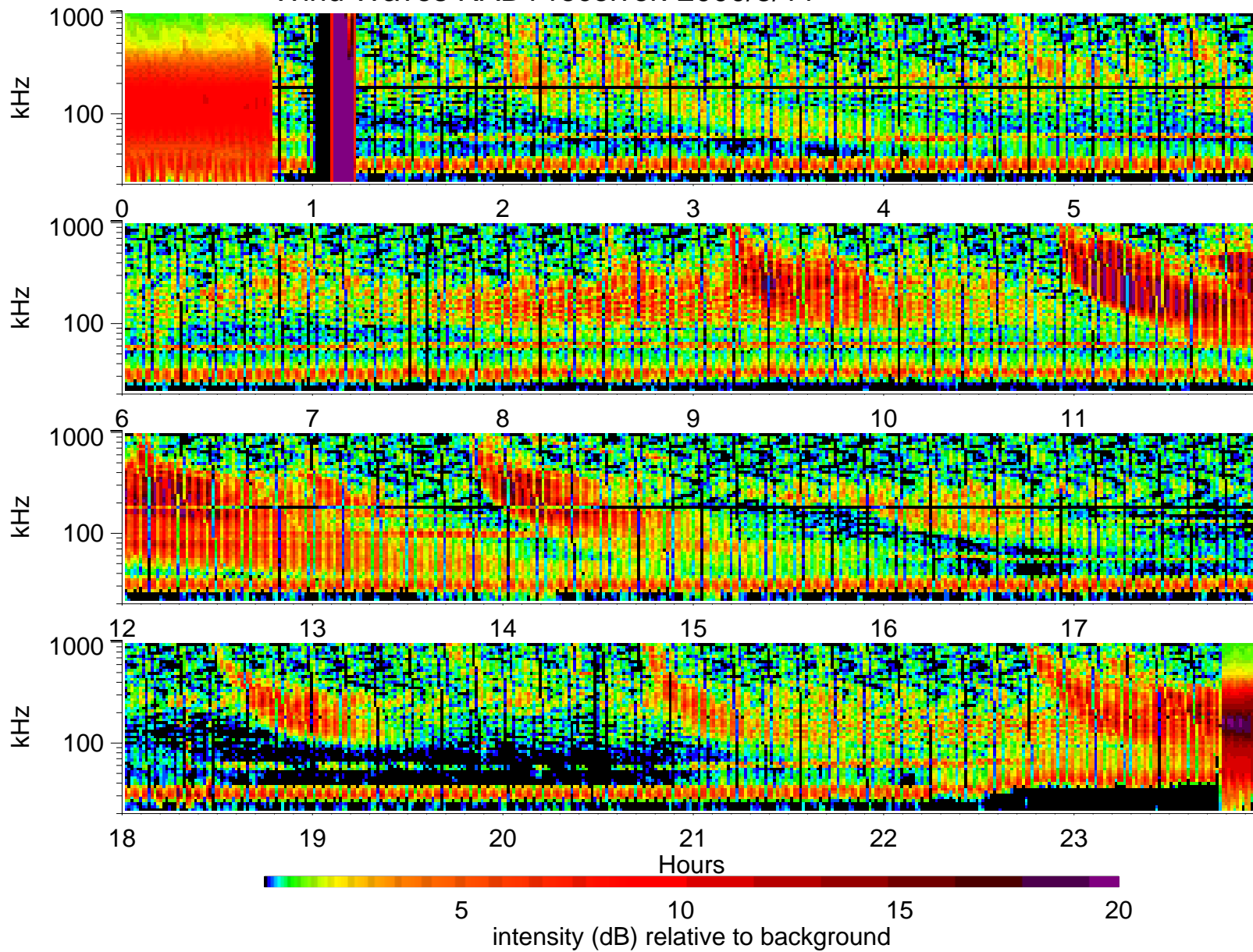
Wind Waves RAD1 receiver: 2000/5/11
