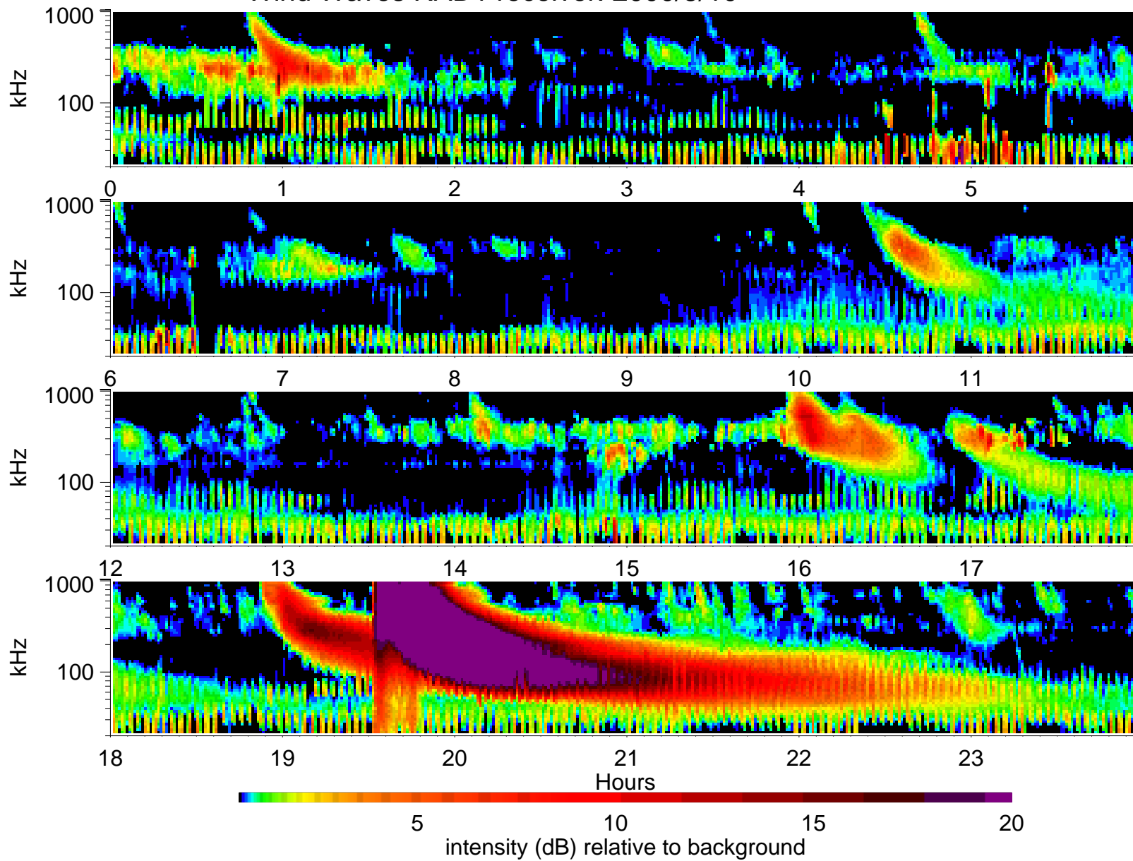
Wind Waves RAD1 receiver: 2000/5/10
