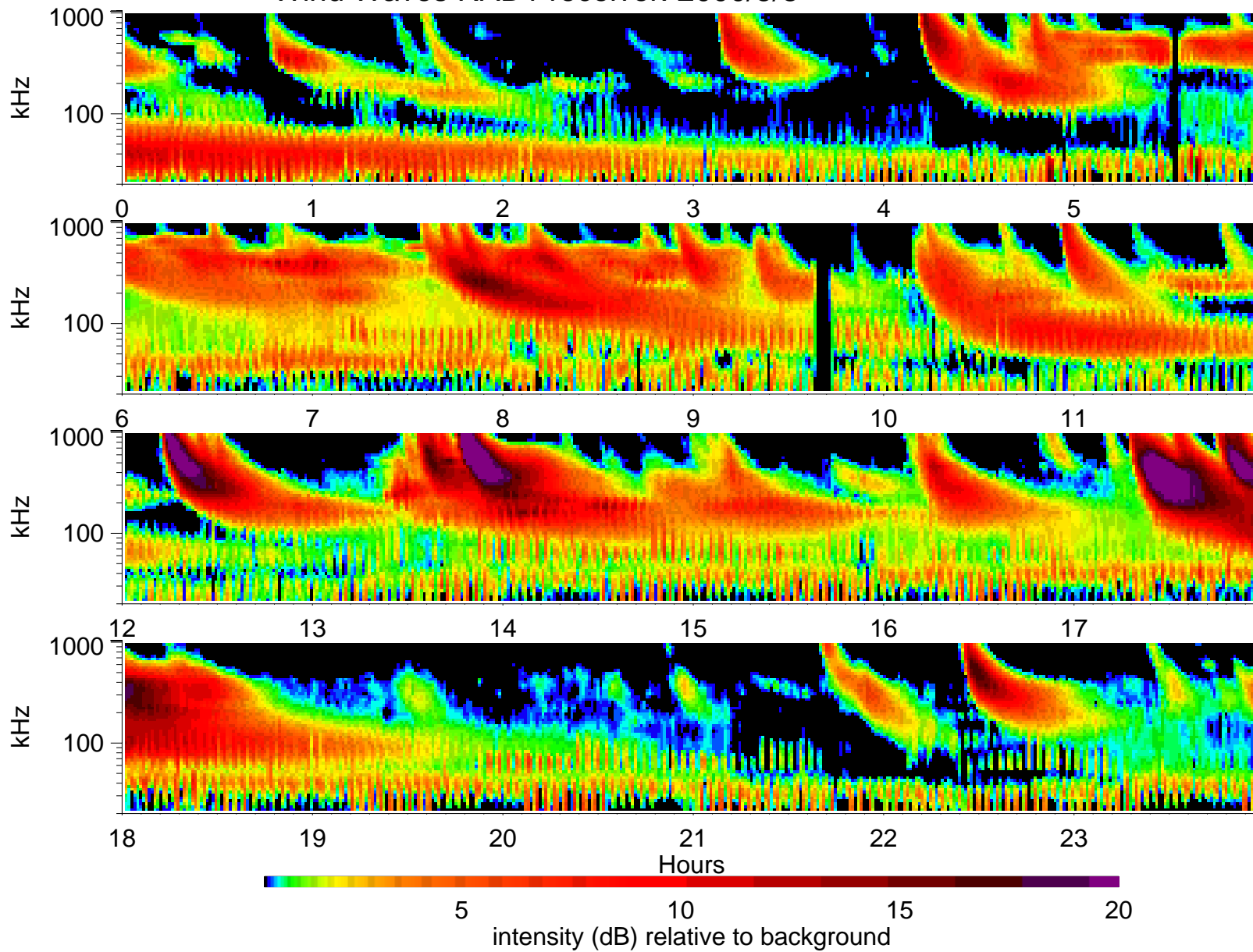
Wind Waves RAD1 receiver: 2000/5/8
