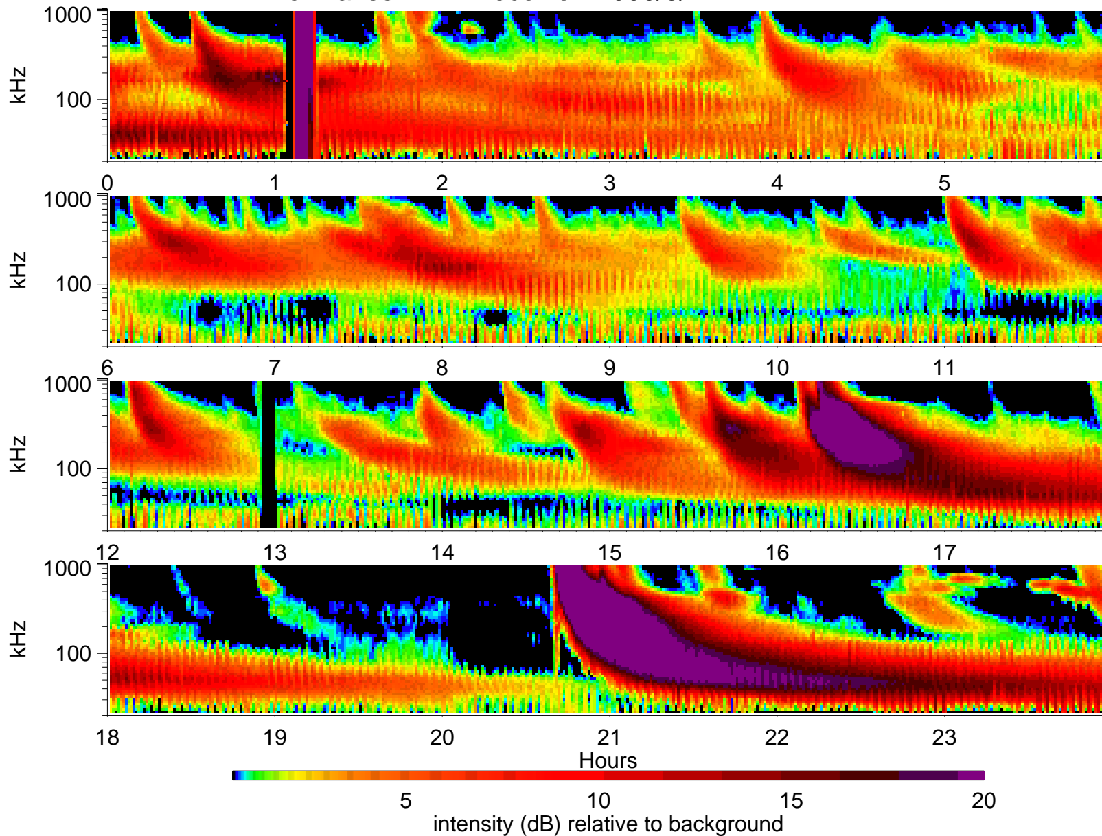
Wind Waves RAD1 receiver: 2000/5/7
