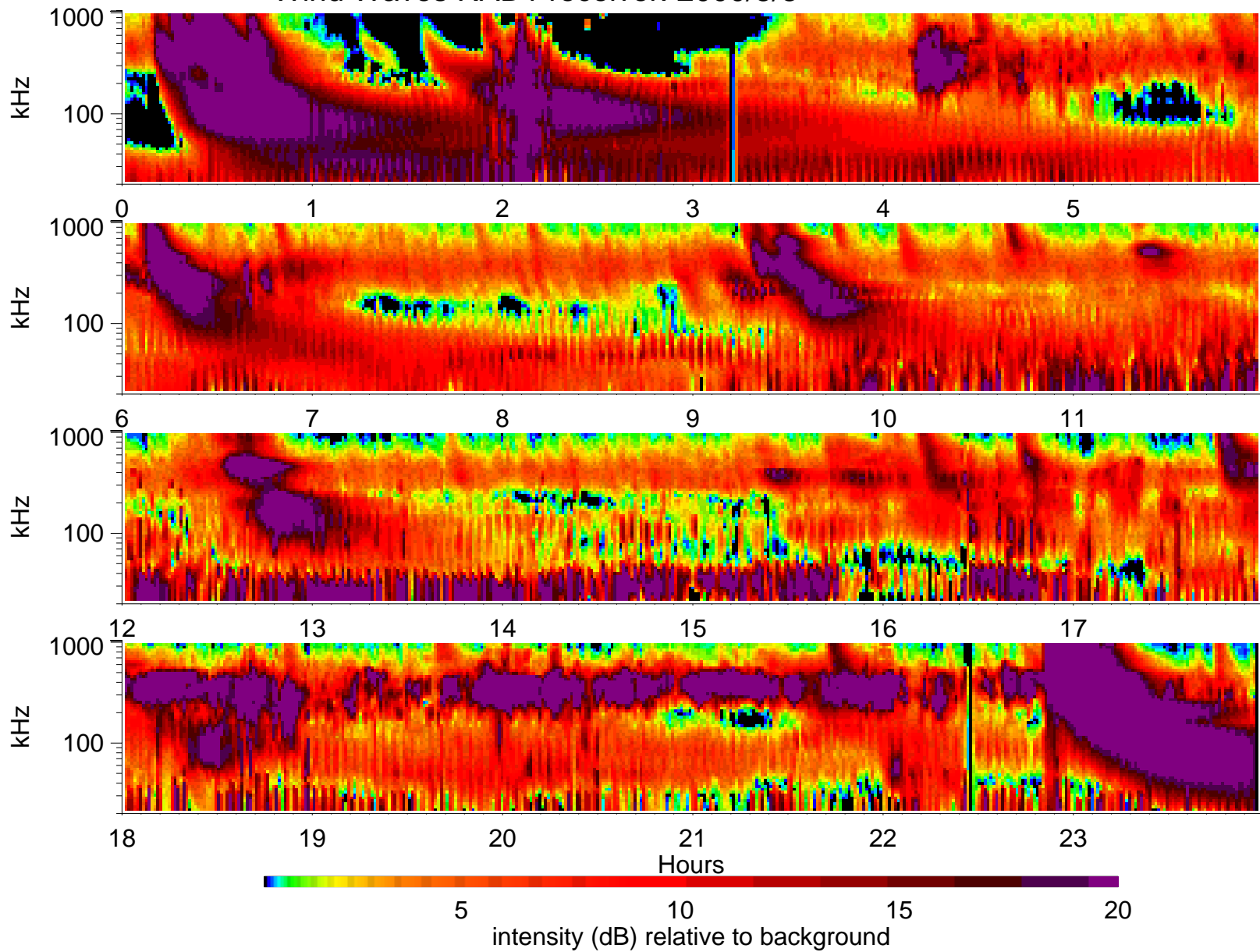
Wind Waves RAD1 receiver: 2000/5/3
