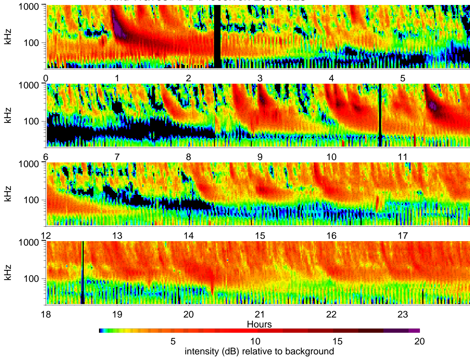
Wind Waves RAD1 receiver: 2000/4/28
