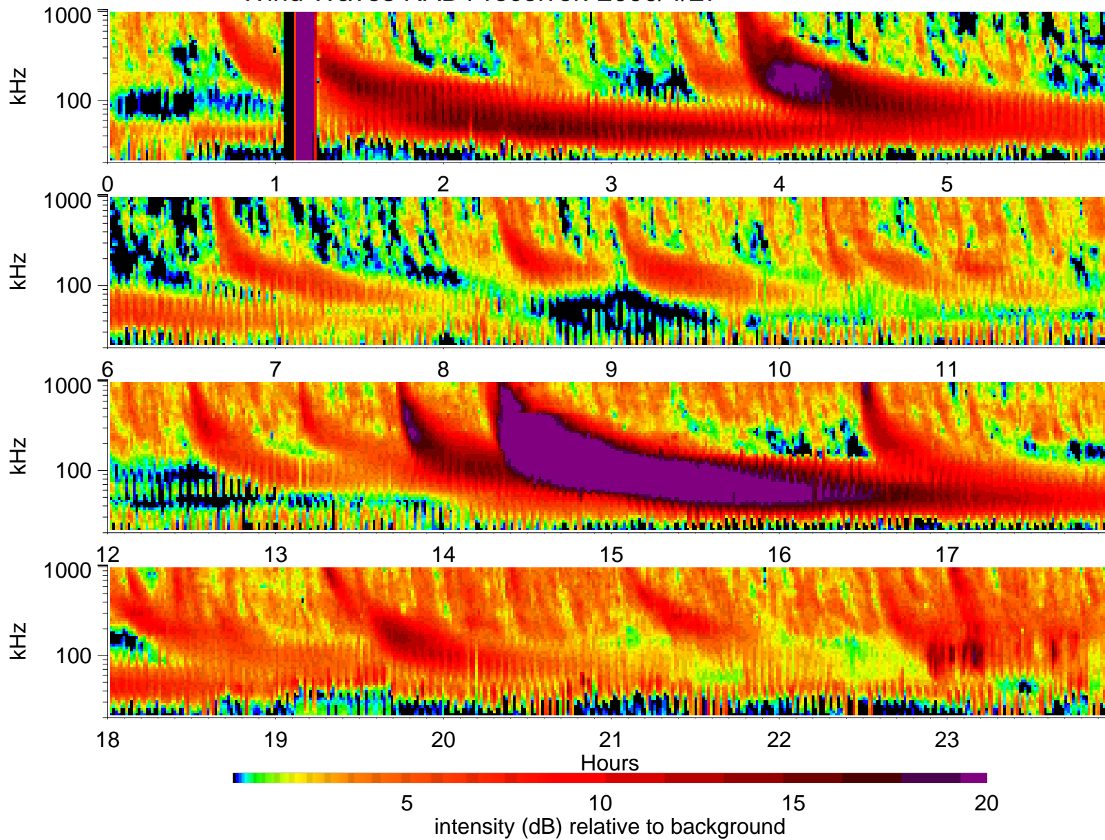
Wind Waves RAD1 receiver: 2000/4/27
