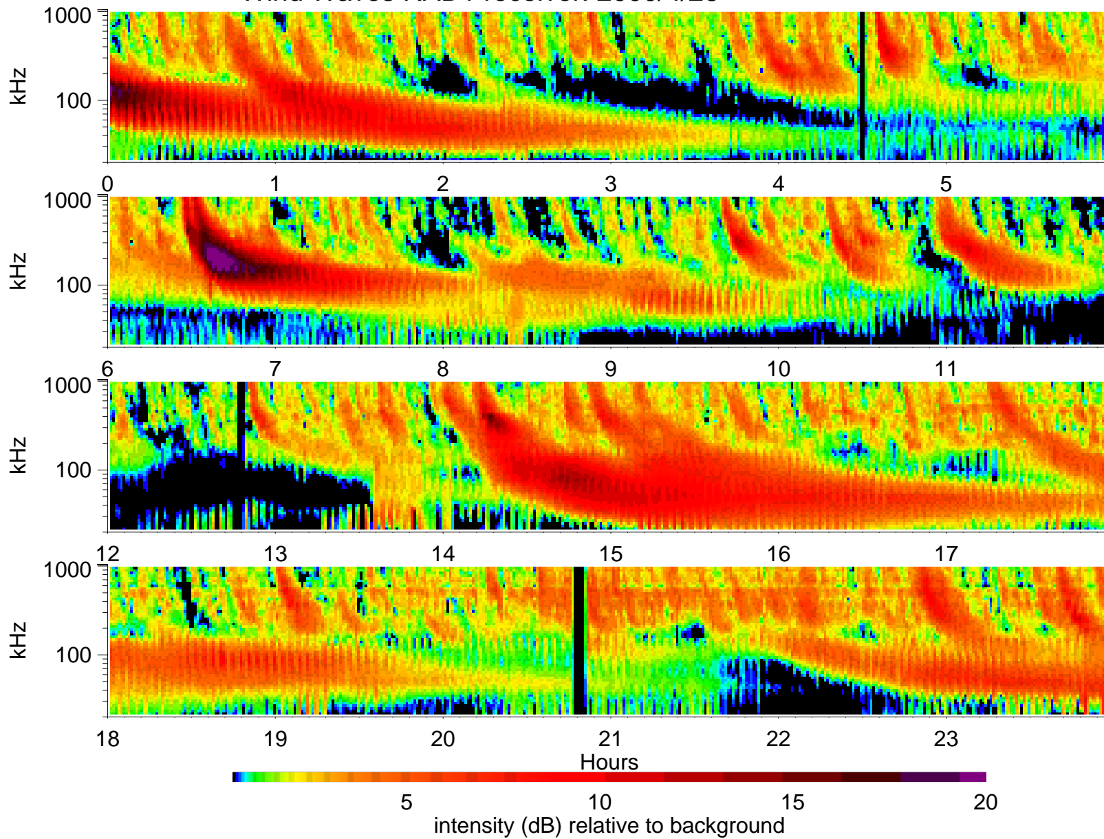
Wind Waves RAD1 receiver: 2000/4/26
