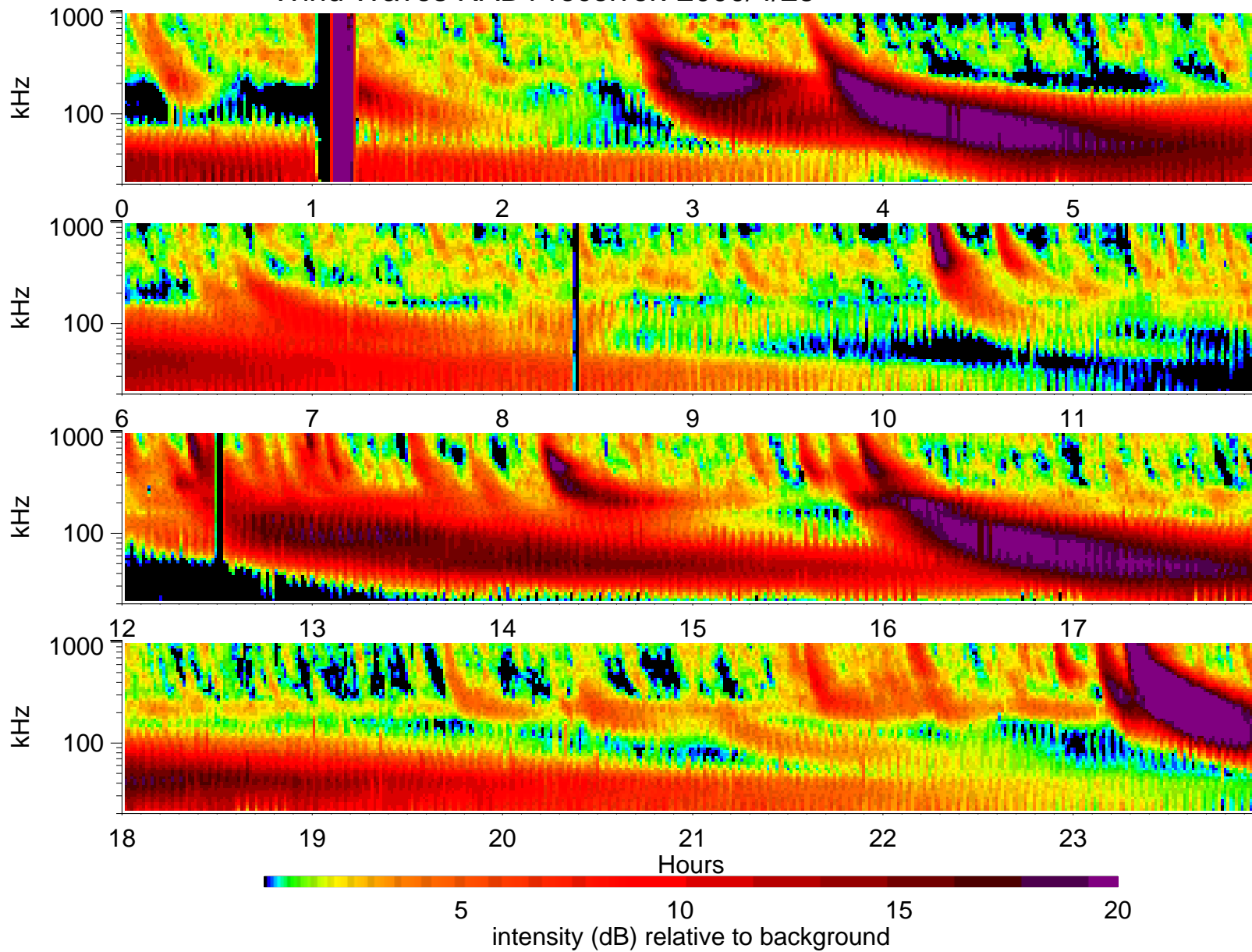
Wind Waves RAD1 receiver: 2000/4/25
