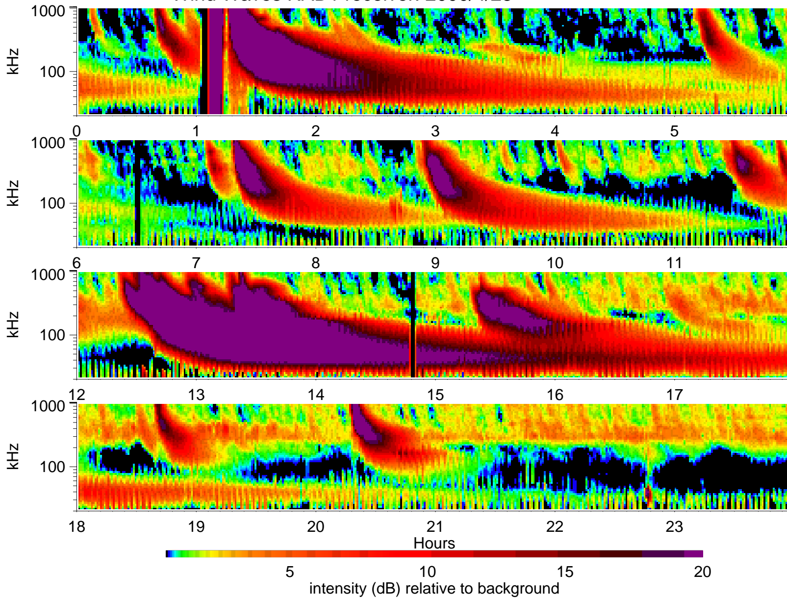
Wind Waves RAD1 receiver: 2000/4/23
