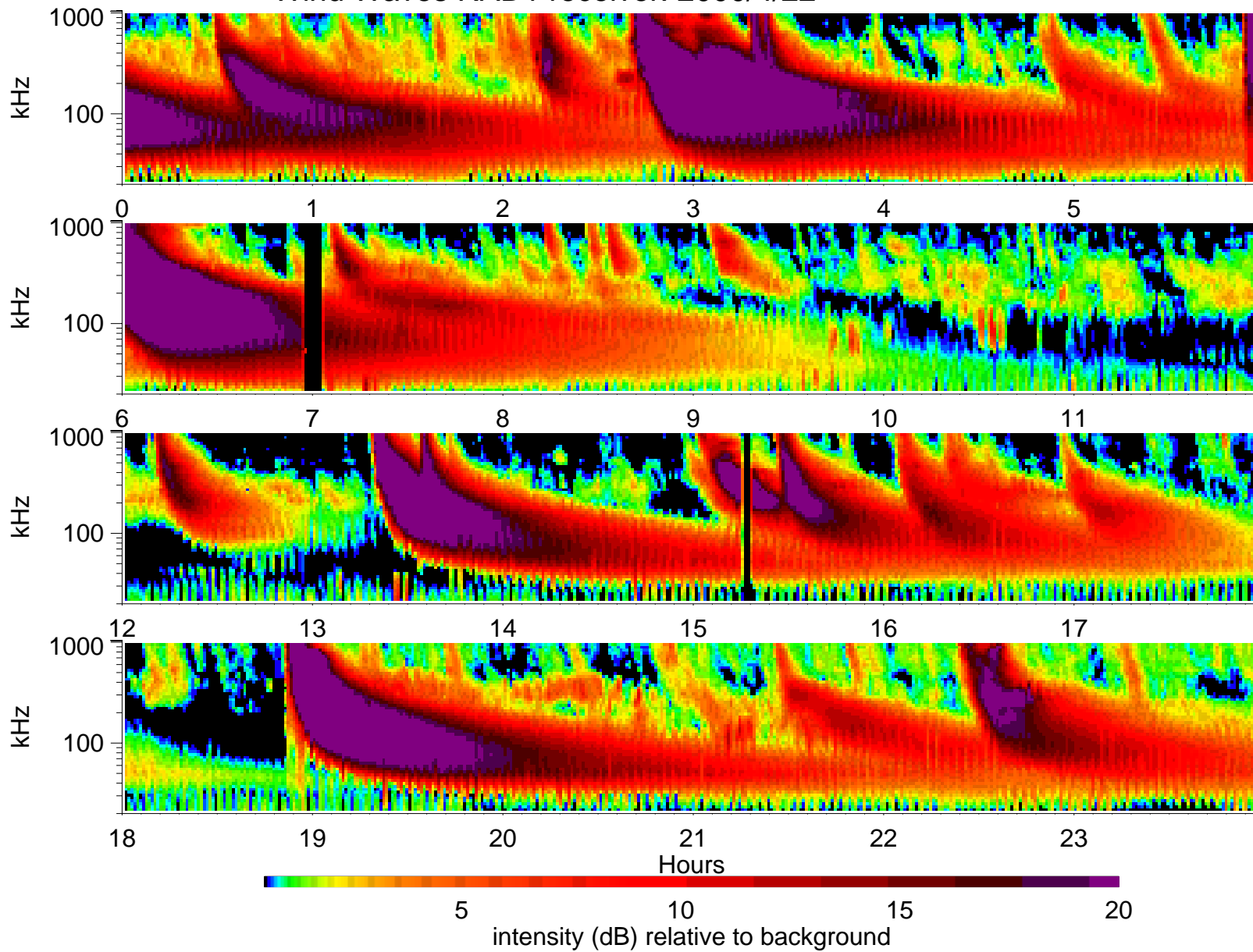
Wind Waves RAD1 receiver: 2000/4/22
