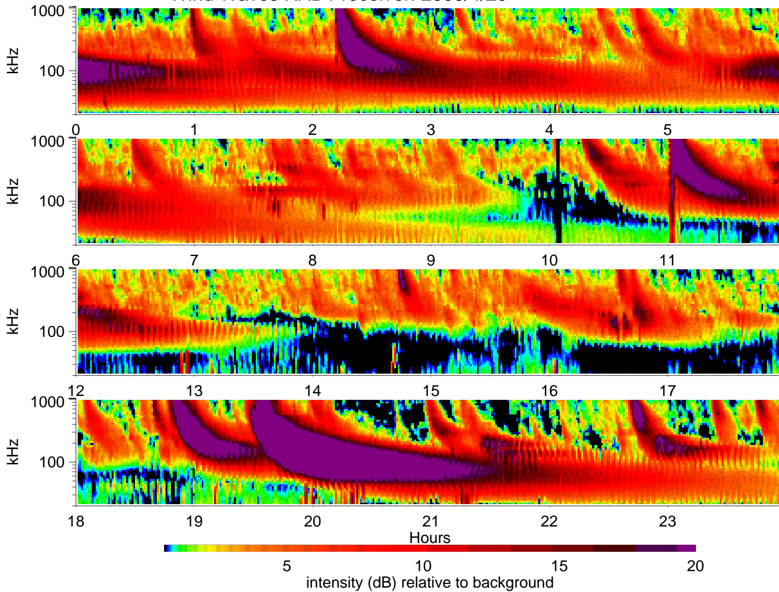
Wind Waves RAD1 receiver: 2000/4/20
