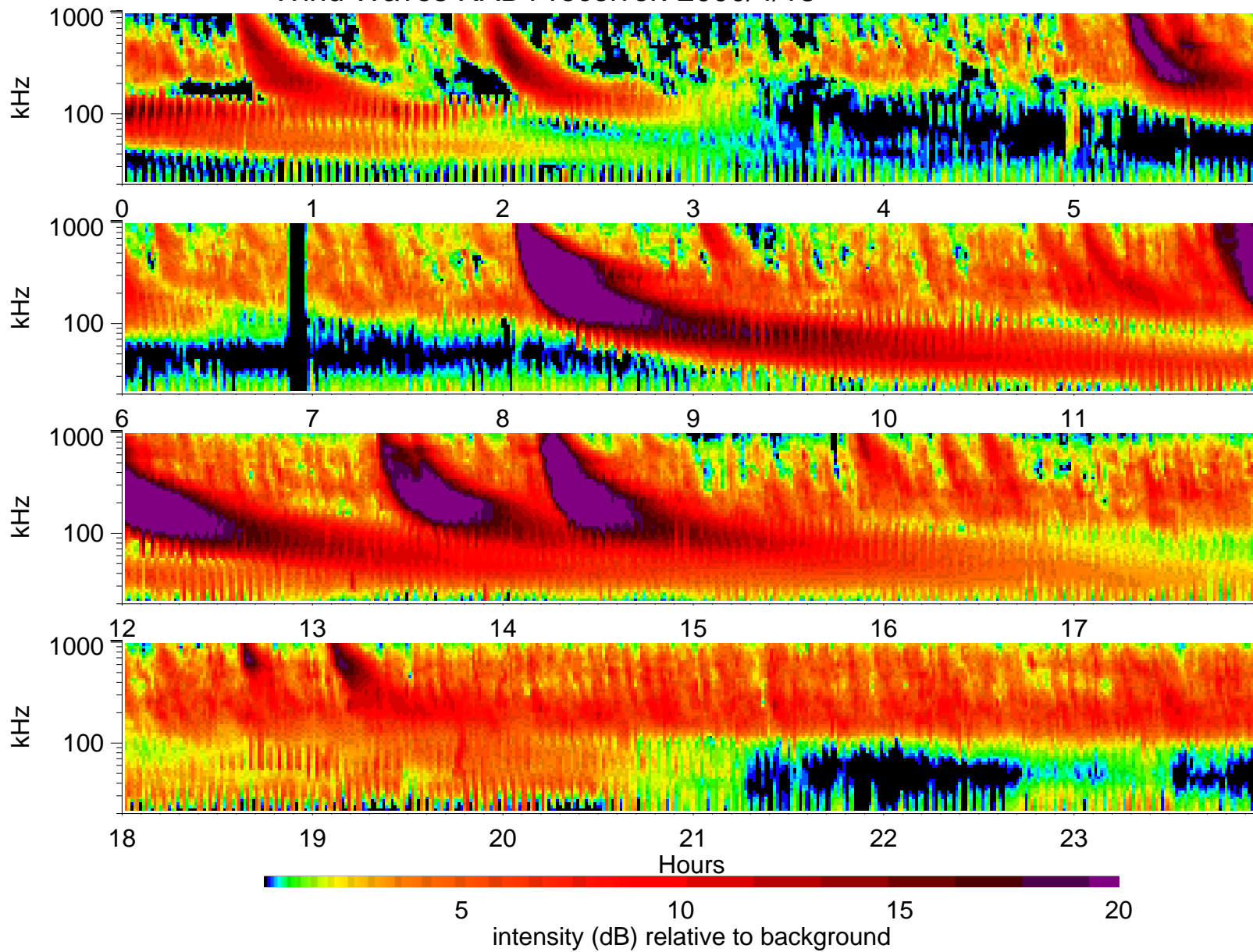
Wind Waves RAD1 receiver: 2000/4/18
