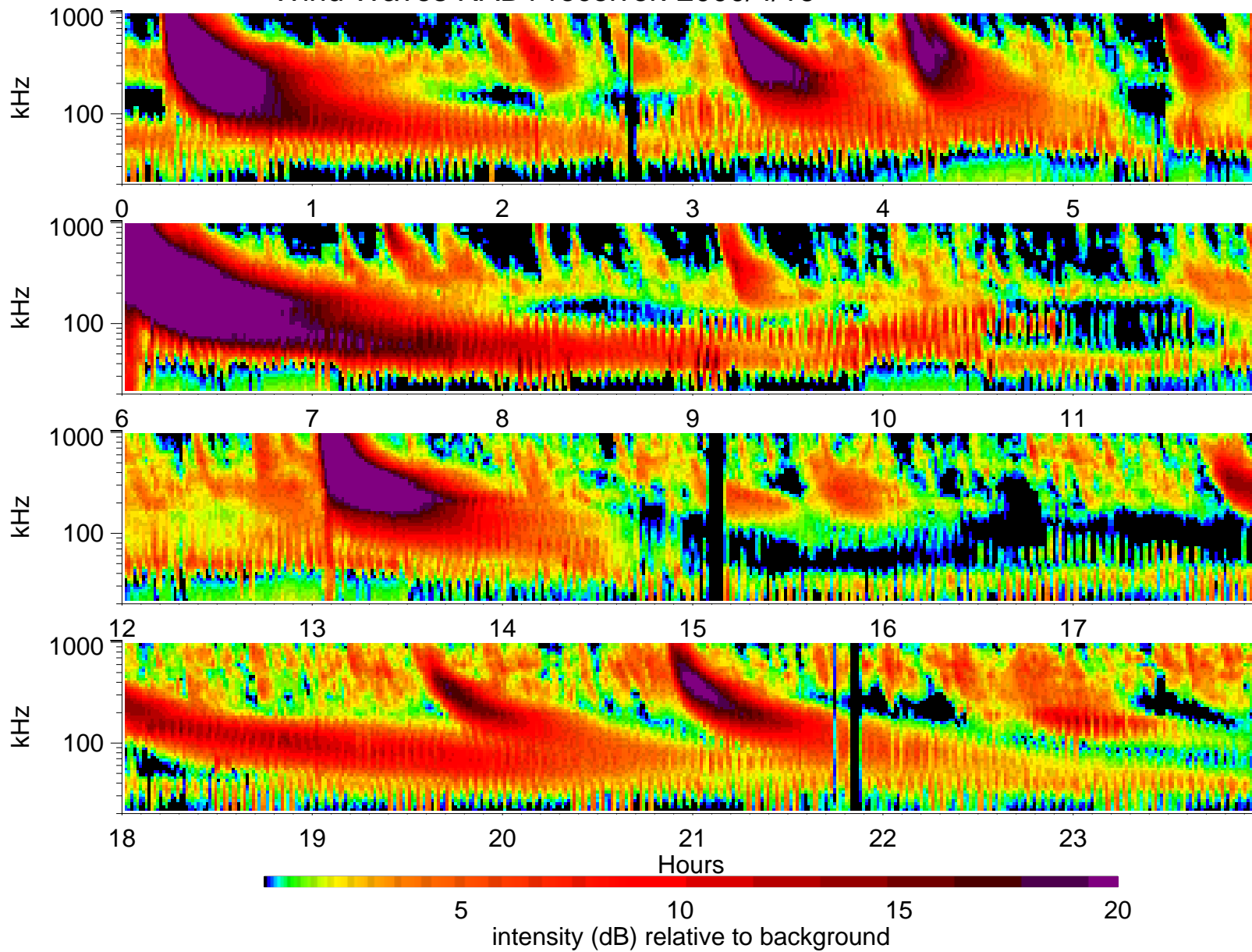
Wind Waves RAD1 receiver: 2000/4/16
