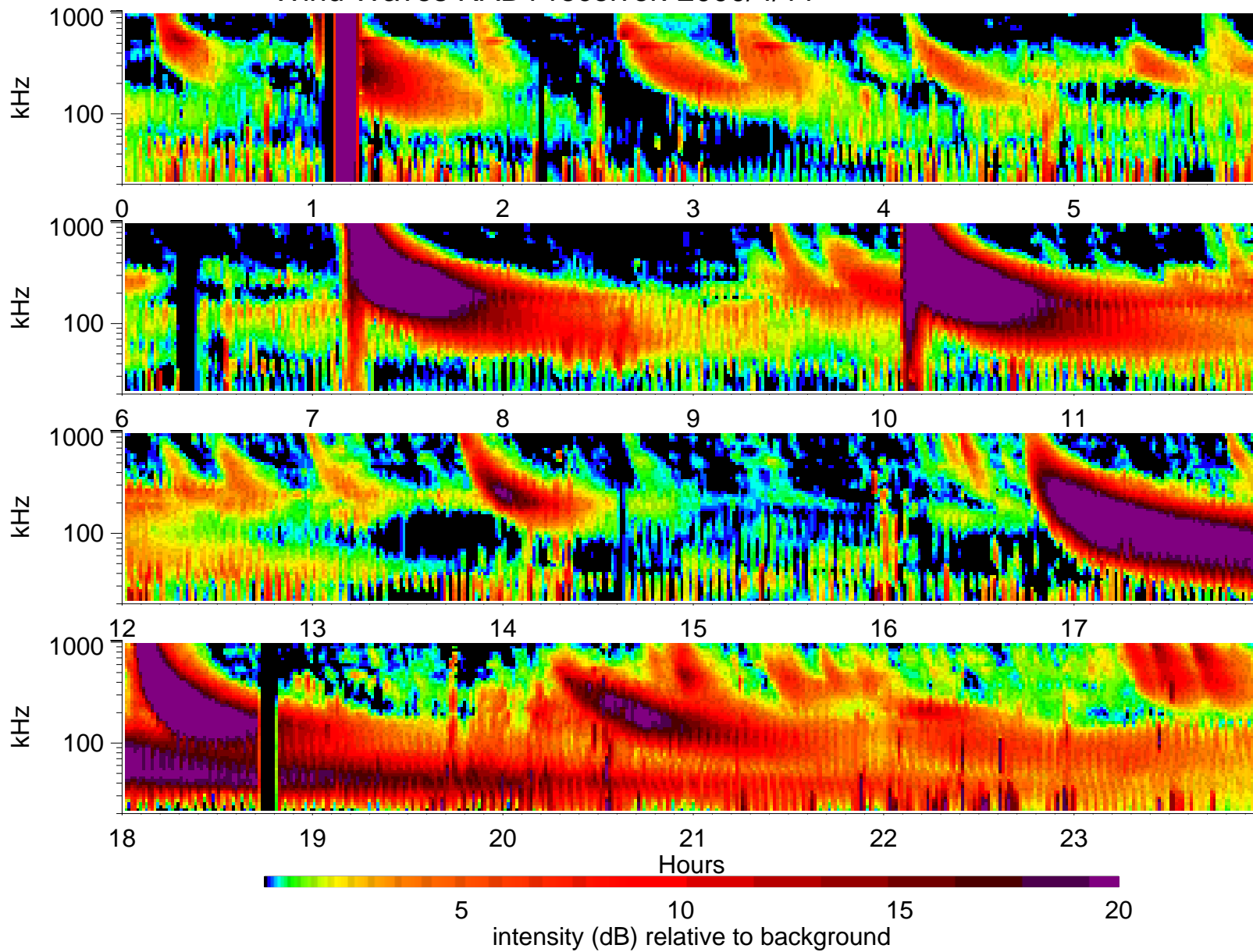
Wind Waves RAD1 receiver: 2000/4/11
