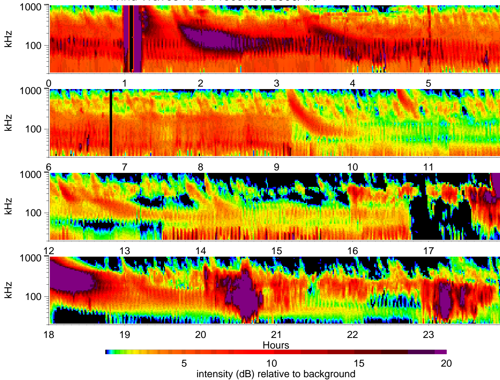
Wind Waves RAD1 receiver: 2000/4/7
