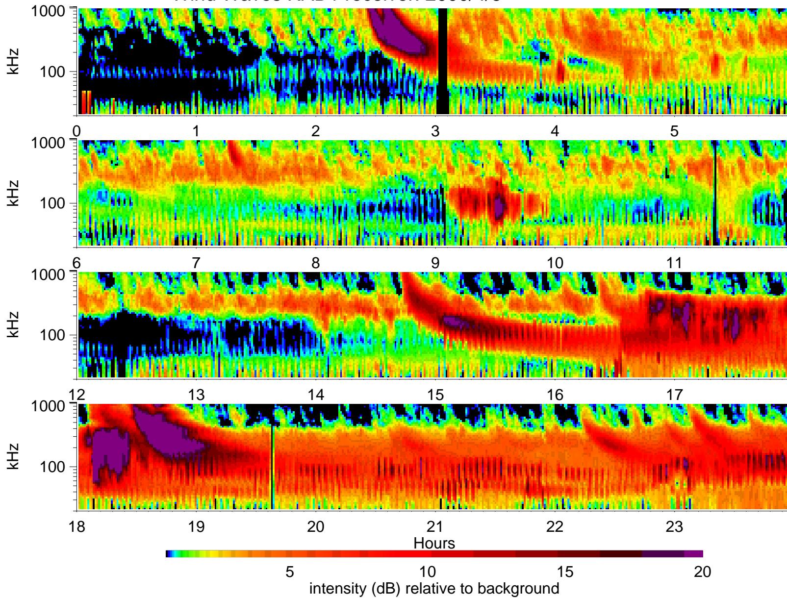
Wind Waves RAD1 receiver: 2000/4/6
