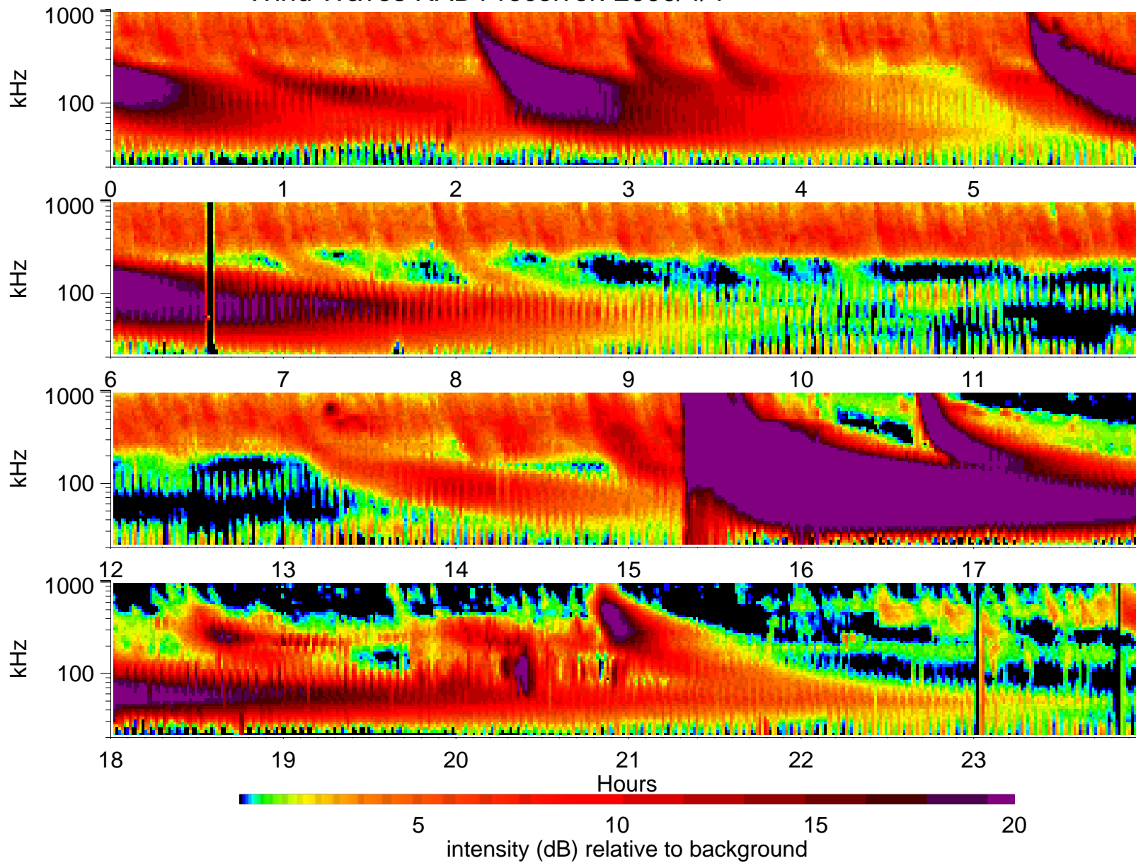
Wind Waves RAD1 receiver: 2000/4/4
