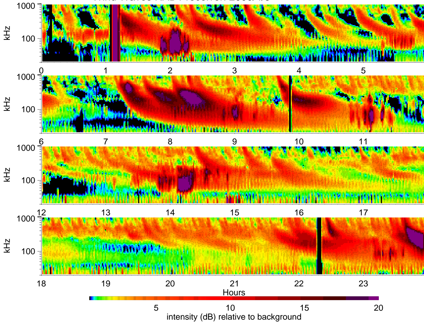
Wind Waves RAD1 receiver: 2000/4/3
