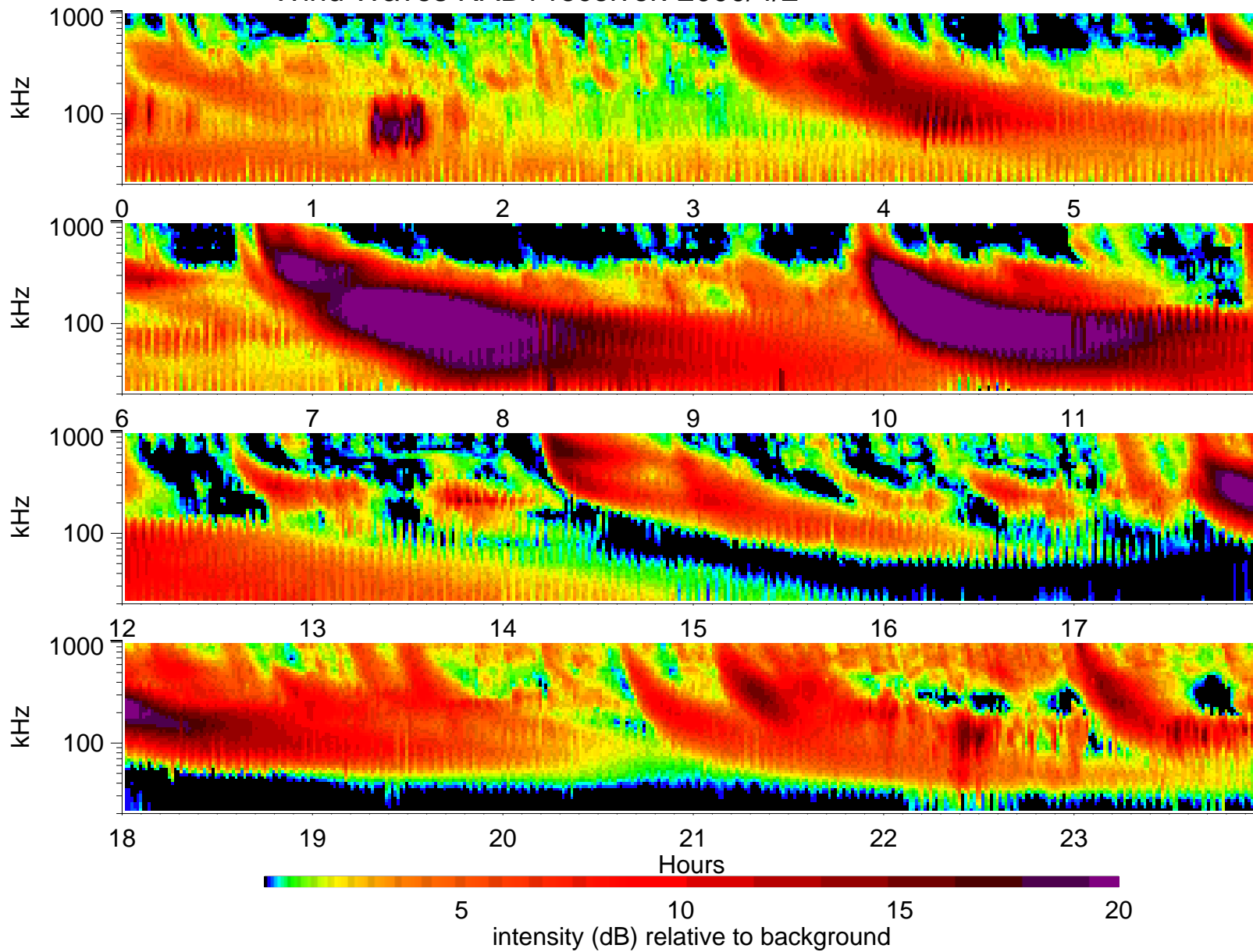
Wind Waves RAD1 receiver: 2000/4/2
