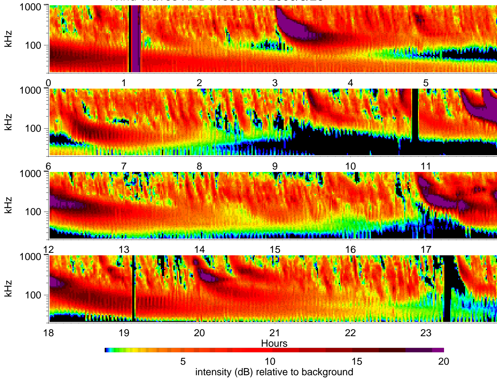
Wind Waves RAD1 receiver: 2000/3/26
