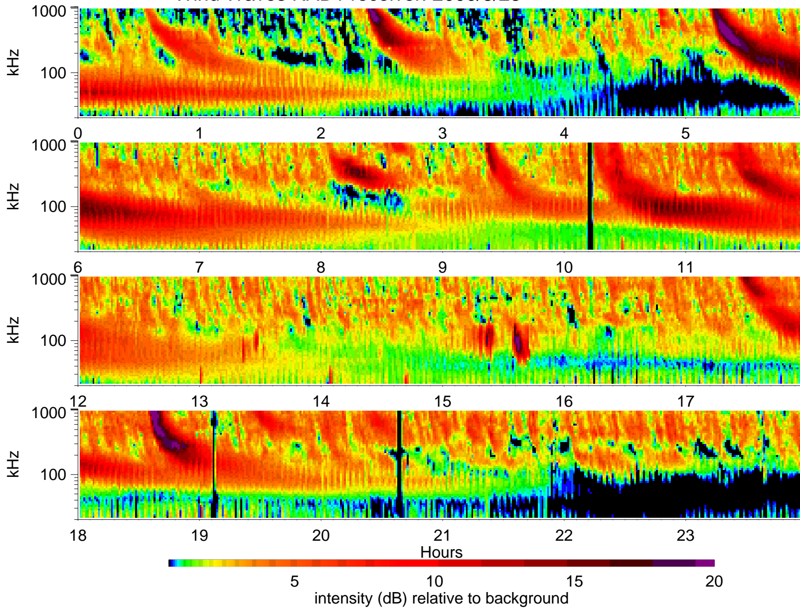
Wind Waves RAD1 receiver: 2000/3/23
