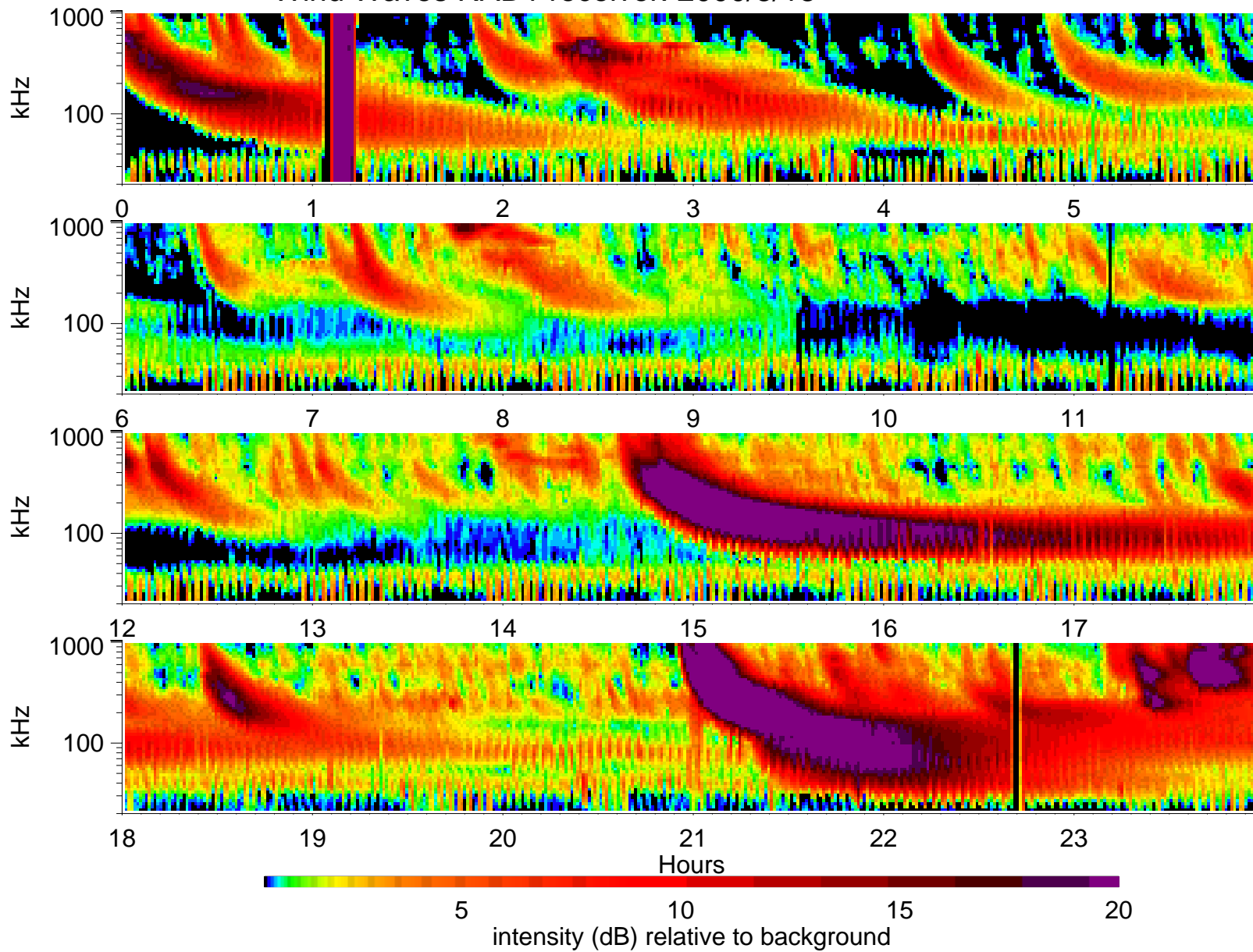
Wind Waves RAD1 receiver: 2000/3/18
