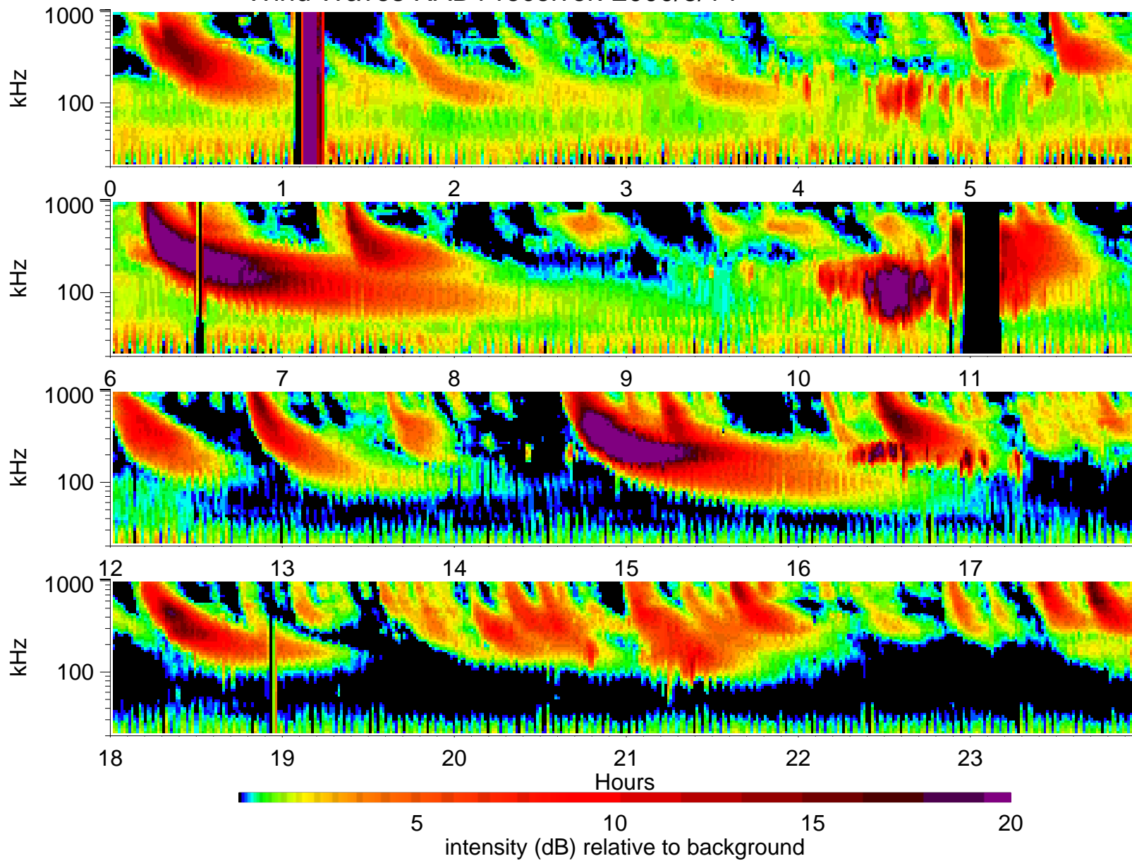
Wind Waves RAD1 receiver: 2000/3/14
