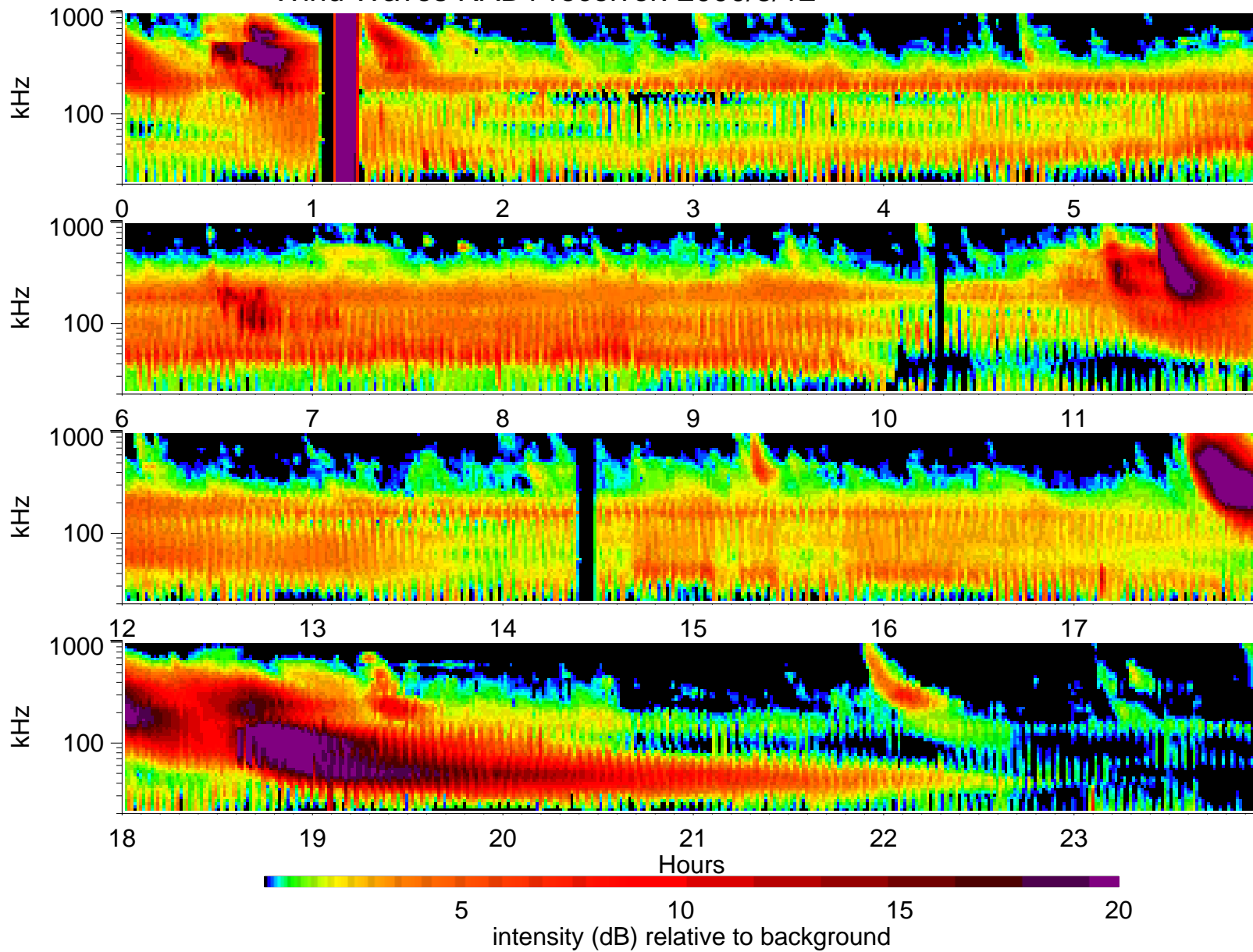
Wind Waves RAD1 receiver: 2000/3/12
