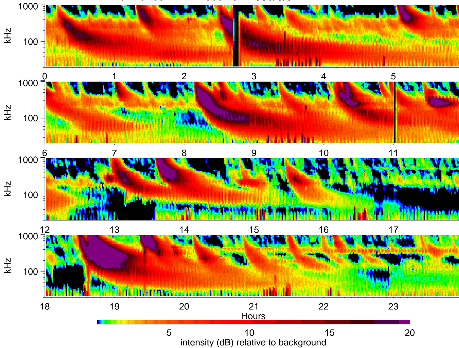
Wind Waves RAD1 receiver: 2000/3/9
