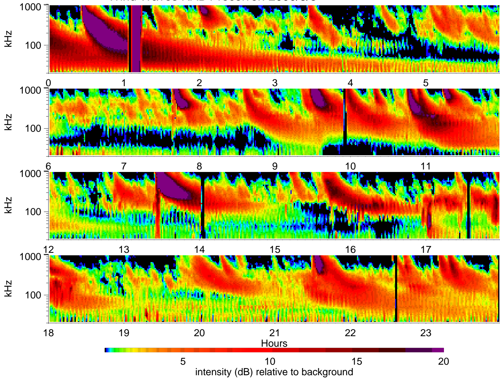
Wind Waves RAD1 receiver: 2000/3/8
